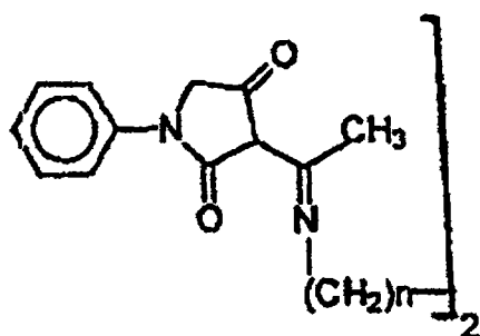
STRUCTURE X
