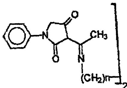
STRUCTURE X
