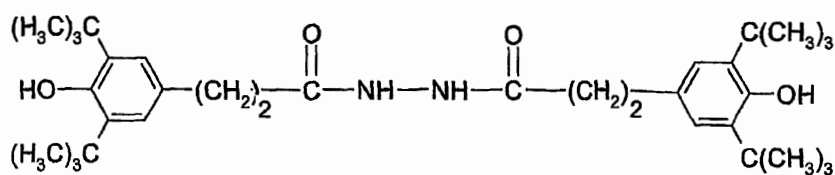
Compound (III-1):
