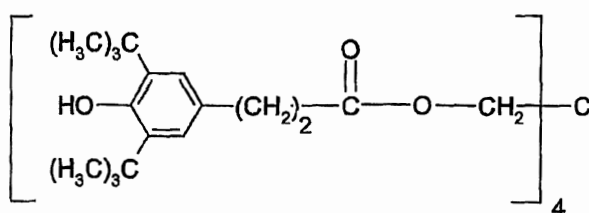
Compound (III-1):
