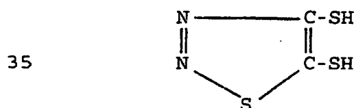
30 4,5-dimercapto-1,2,3-thiadiazole
