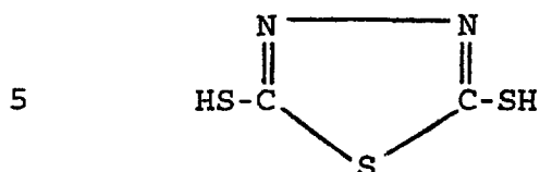
2,5-dimercapto-1,3,4-thiadiazole
