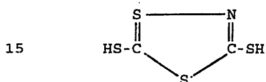
20 3,4-dimercapto-1,2,5-thiadiazole
