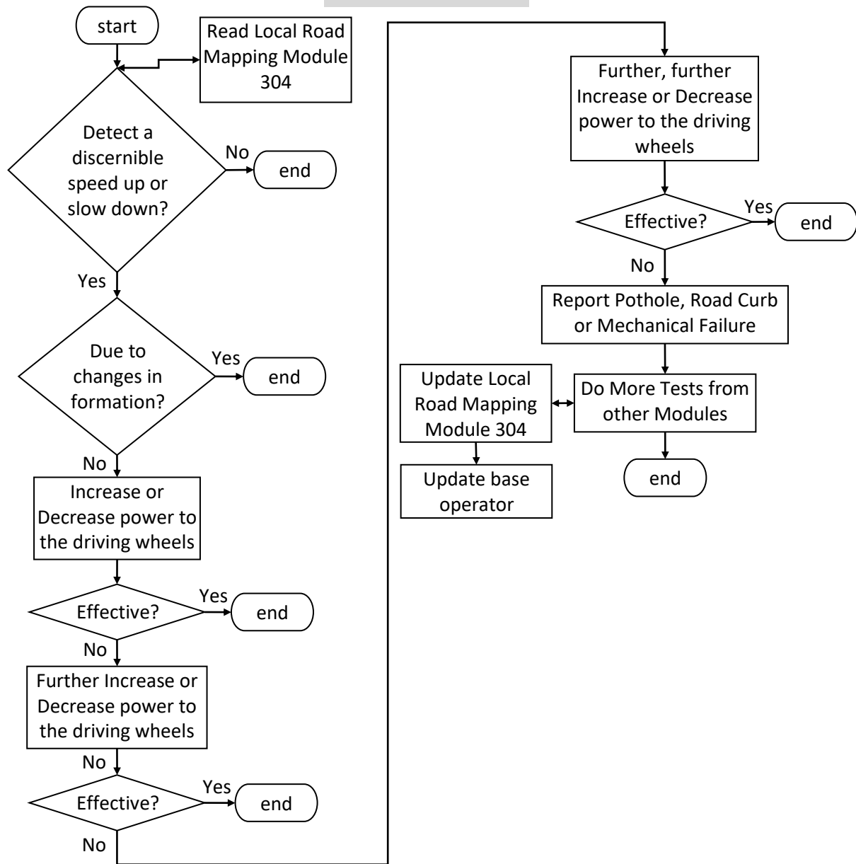
FIGURE 7: A Sample Automatic Gradient Detection Flow Chart
