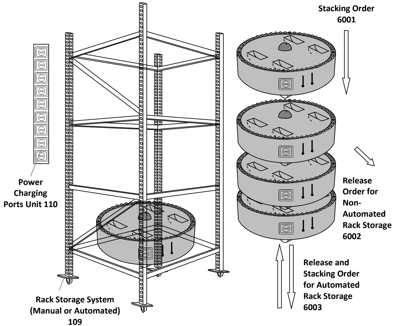
FIGURE 9: A Sample Manual or Automated Rack Storage System with Power Charging Ports Unit
