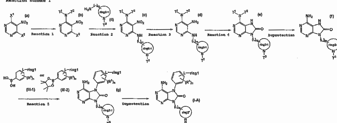
Reaction scheme 1
