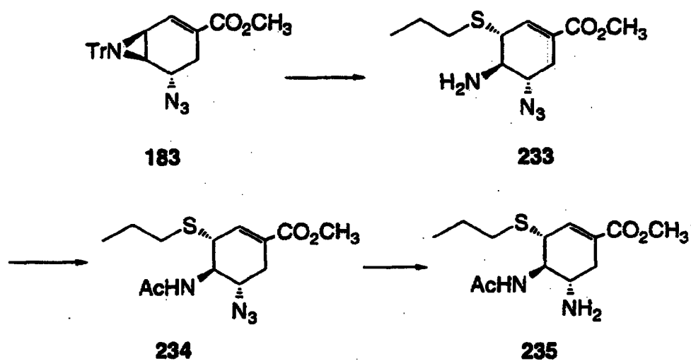
Scheme 30
