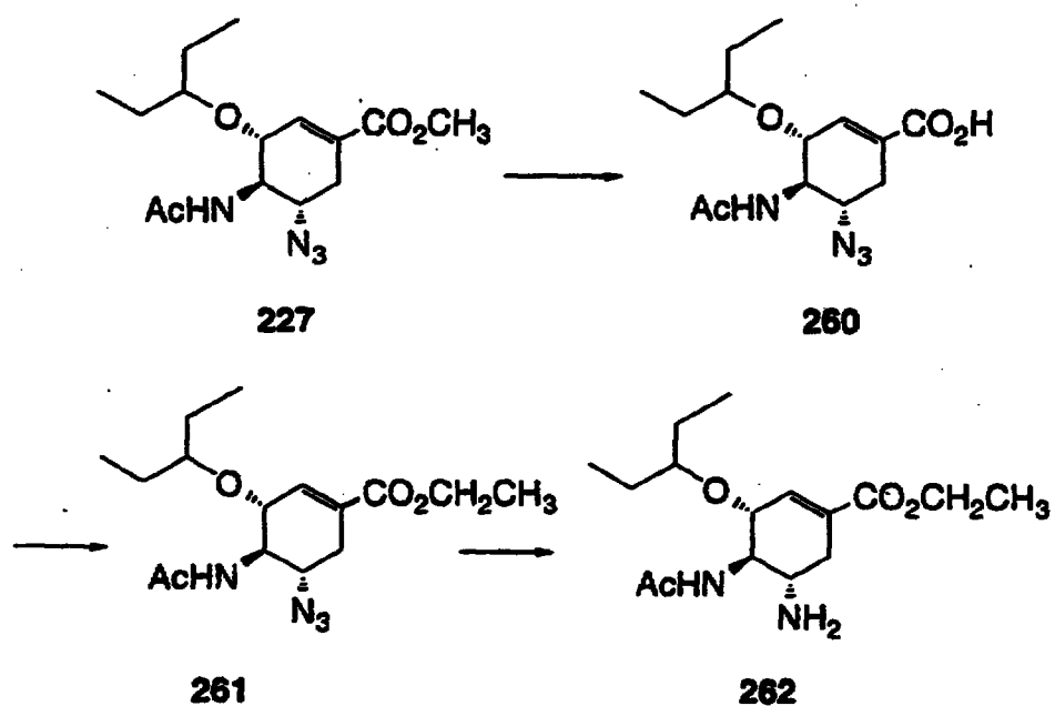
Scheme 34
