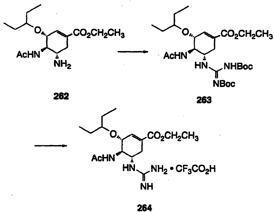
Scheme 35
