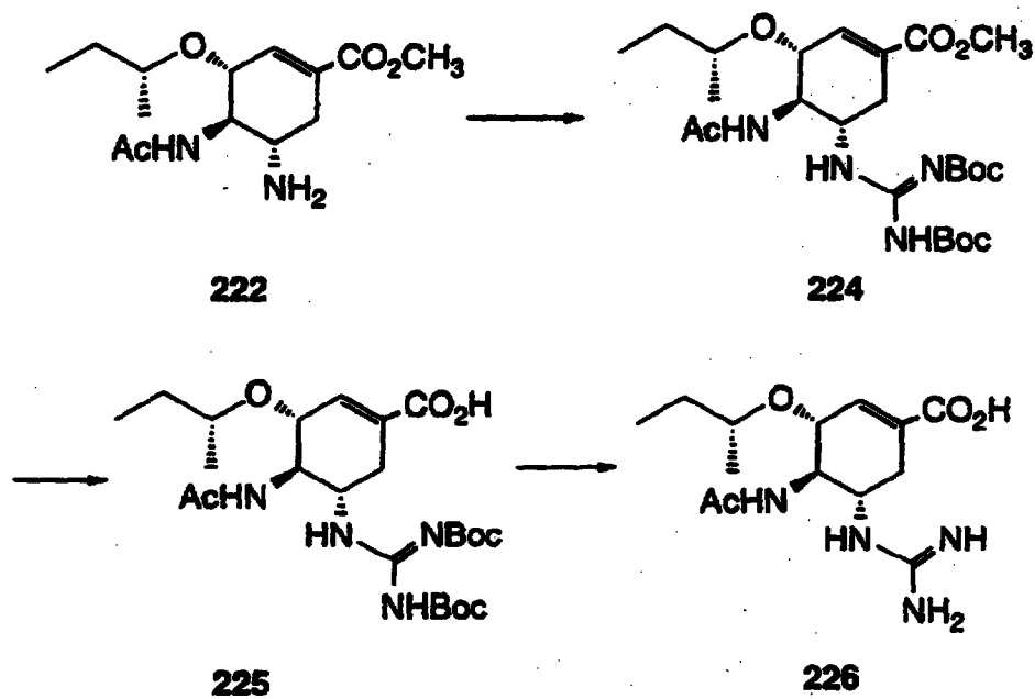
Scheme 27
