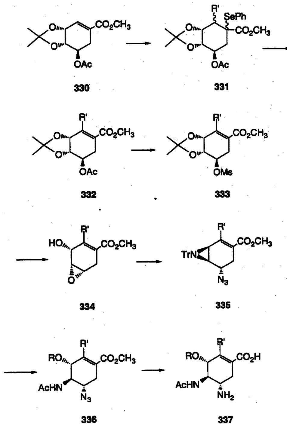
Scheme 43
