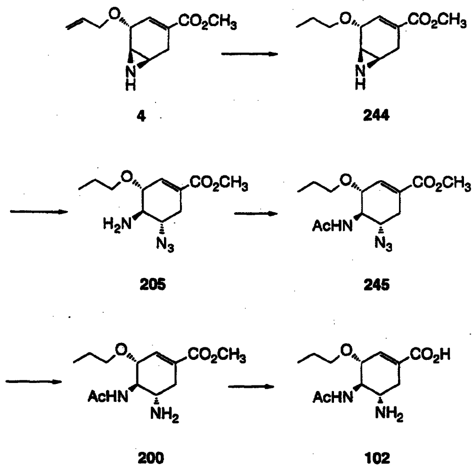
Scheme 32
