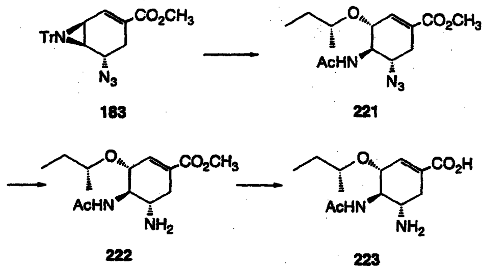
Scheme 26
