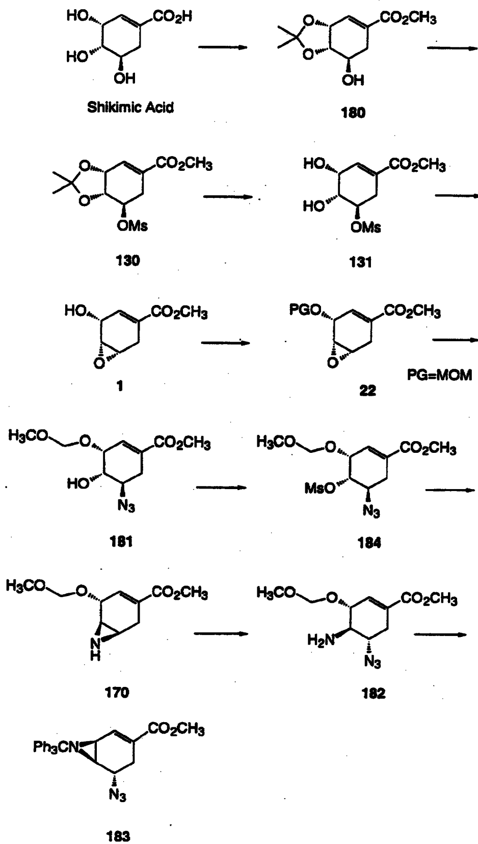
Scheme 17
