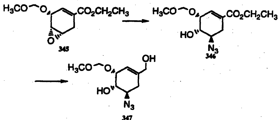
5 Scheme 45
