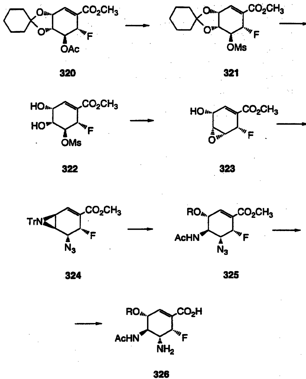
Scheme 42
