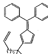
2-(1,1-dimethylpent-4-enyl)-6,6-diphenylpentafulvene
