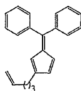
2-(pent-4-enyl)-6,6-diphenylpentafulvene
