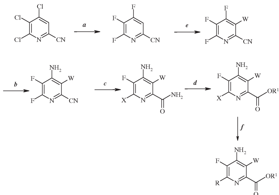
Scheme IV
