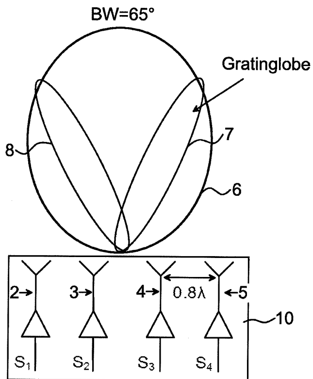
Fig. 1 (PRIOR ART)
