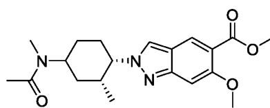
And Enantiomer
