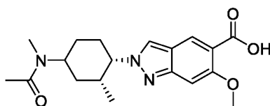
And Enantiomer
