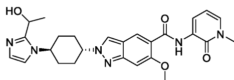
ISOMER 1
