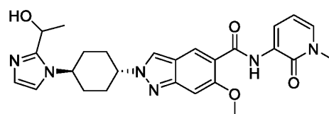
ISOMER 2
