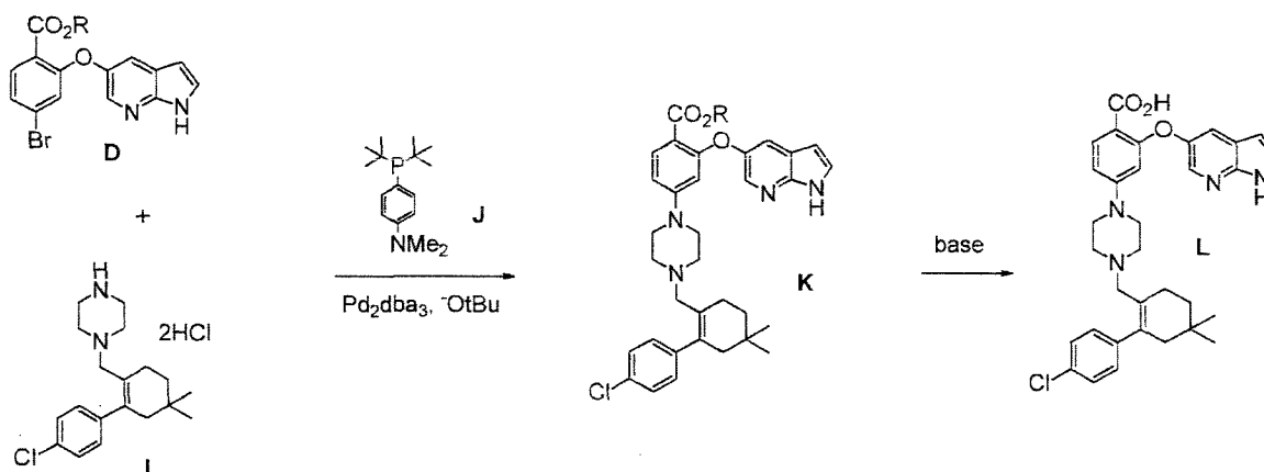
Scheme 5
