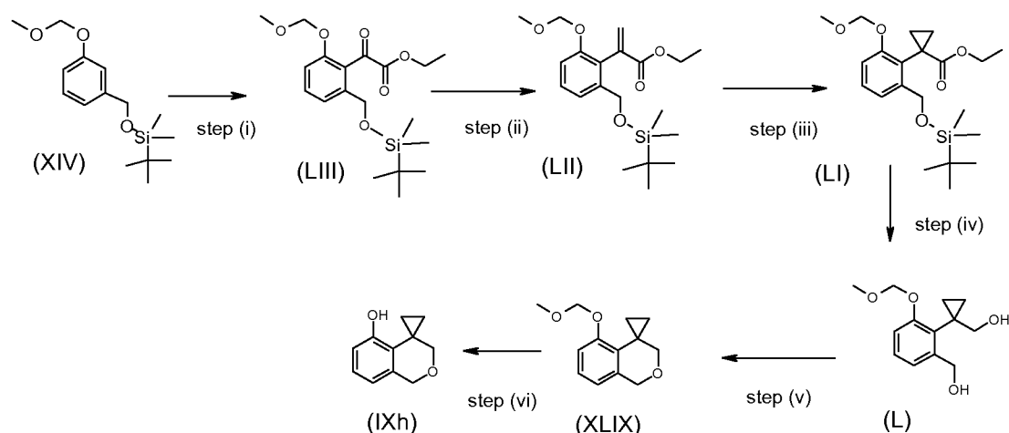
Scheme 19a
