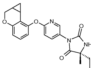
diastereoisomer 1
