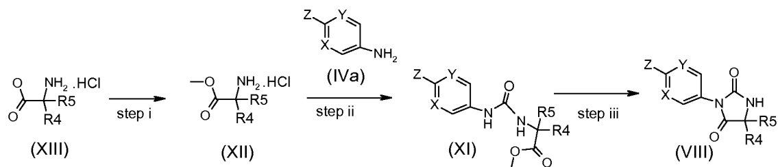
Scheme 26
