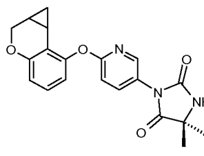
diastereoisomer 2
