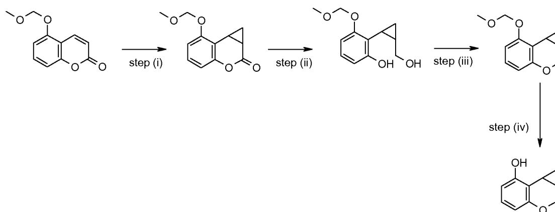
Scheme 18b
