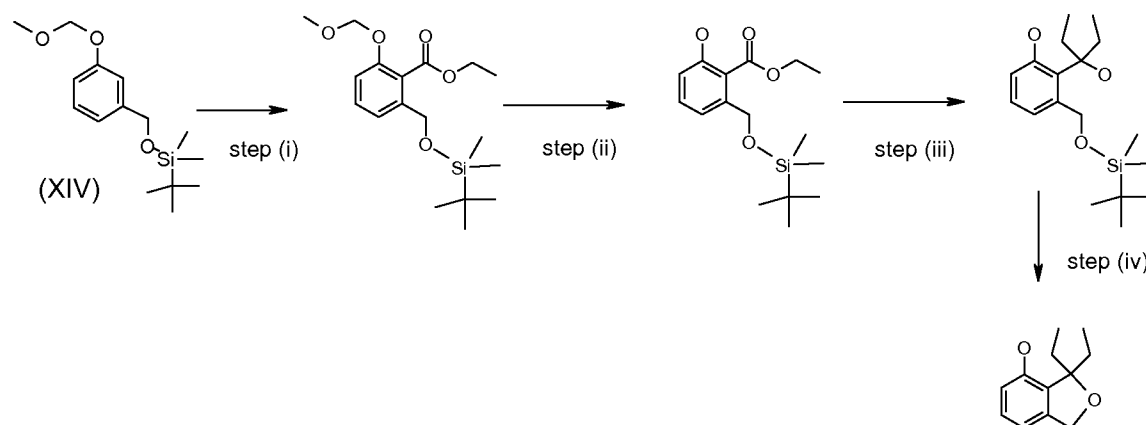
Scheme 19b
