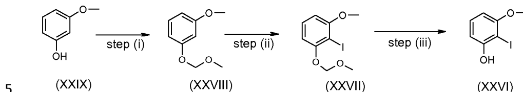
Scheme 14
