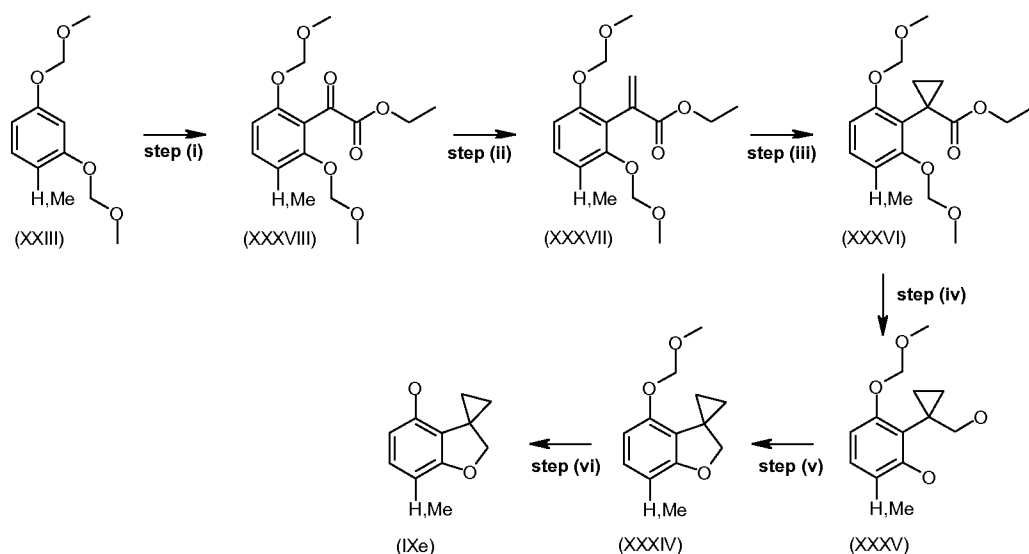
Scheme 16
