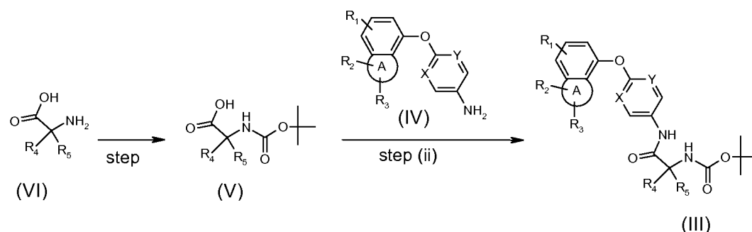
Scheme 2b
