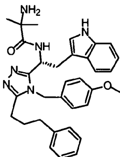
compound 23 ( R )- N -(1-(5-(3-(1 H -indol-3-yl)propyl)-4-(4-methoxybenzyl)-4 H -1,2,4-triazol-3-yl)-2-(1 H -indol-3-yl)ethyl)-2-amino-2-methylpropanamide,
