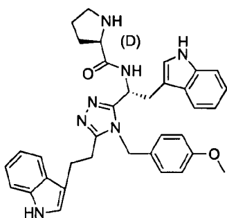
compound 91 (R)-N-(1-(5-(2-(1H-indol-3-yl)ethyl)-4-(4-methoxybenzyl)-4H-1,2,4-triazol-3-yl)-2-(1H-indol-3-yl)ethyl)-2-(pyridin-2-yl)acetamide,
