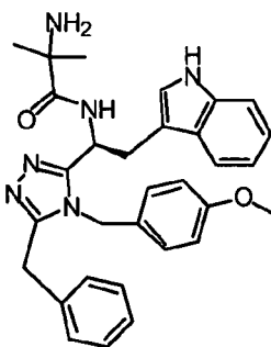
compound 128 N-((R)-1-(4-(4-nitrobenzyl)-5-phenethyl-4H-1,2,4-triazol-3-yl)-2-(1H-indol-3-yl)ethyl)-2-amino-2-methylpropanamide,
