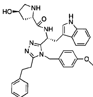
5 compound 41 ( S )- N -(( R )-1-(4-(4-methoxybenzyl)-5-phenethyl-4 H -1,2,4-triazol-3-yl)-2-(1 H -indol-3-yl)ethyl)piperidine-3-carboxamide,
