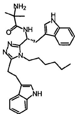
5 compound 16 ( R )- N -(1-(5-(3-(1 H -indol-3-yl)propyl)-4-hexyl-4 H -1,2,4-triazol-3-yl)-2-(1 H -indol-3-yl)ethyl)-2-amino-2-methylpropanamide,
