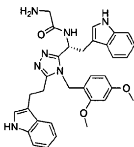
compound 70 (S)-N-((R)-1-(5-(2-(1H-indol-3-yl)ethyl)-4-(2,4-dimethoxybenzyl)-4H-1,2,4-triazol-3-yl)-2-(1H-indol-3-yl)ethyl)pyrrolidine-2-carboxamide,
