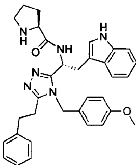
5 compound 47 (R)-N-((R)-1-(4-(4-methoxybenzyl)-5-phenethyl-4H-1,2,4-triazol-3-yl)-2-(1H-indol-3-yl)ethyl)pyrrolidine-2-carboxamide,
