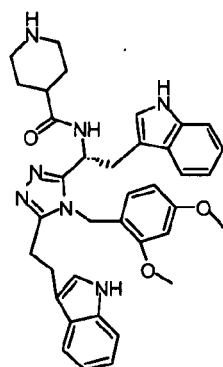
compound 32 ( R )- N -(1-(5-(2-(1 H -indol-3-yl)ethyl)-4-(2,4-dimethoxybenzyl)-4 H -1,2,4-triazol-3-yl)-2-(1 H -indol-3-yl)ethyl)piperidine-3-carboxamide,
