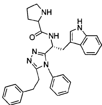
compound 144 N-((R)-2-(1H-indol-3-yl)-1-(5-phenethyl-4-phenyl-4H-1,2,4-triazol-3-yl)ethyl)-2-aminoacetamide,
