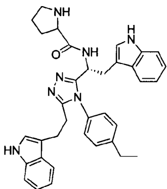
5 compound 152 N-((R)-1-(5-(2-(1H-indol-3-yl)ethyl)-4-(4-methoxybenzyl)-4H-1,2,4-triazol-3-yl)-2-(1H-indol-3-yl)ethyl)-2-aminoacetamide,
