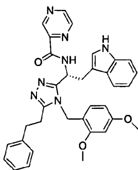
compound 67 ( R )- N -1-(4-(2,4-dimethoxybenzyl)-5-phenethyl-4 H -1,2,4-triazol-3-yl)-2-(1 H -indol-3-yl)ethyl)piperazine-2-carboxamide,
