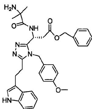
compound 172 N-((R)-1-(5-benzyl-4-((pyridin-3-yl)methyl)-4H-1,2,4-triazol-3-yl)-2-(1H-indol-3-yl)ethyl)-2-amino-2-methylpropanamide,
