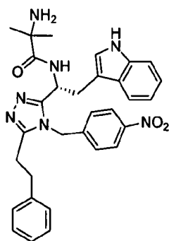
compound 129 (S)-N-(1-(4-(4-methoxybenzyl)-5-phenethyl-4H-1,2,4-triazol-3-yl)-2-(1H-indol-3-yl)ethyl)-2-amino-2-methylpropanamide,
