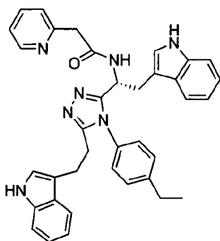
compound 149 N-((R)-1-(5-(2-(1H-indol-3-yl)ethyl)-4-(4-ethylphenyl)-4H-1,2,4-triazol-3-yl)-2-(1H-indol-3-yl)ethyl)-2-aminoacetamide,
