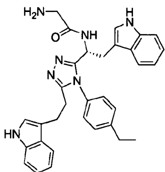
compound 150 (2S)-N-((R)-1-(5-(2-(1H-indol-3-yl)ethyl)-4-(4-ethylphenyl)-4H-1,2,4-triazol-3-yl)-2-(1H-indol-3-yl)ethyl)pyrrolidine-2-carboxamide,
