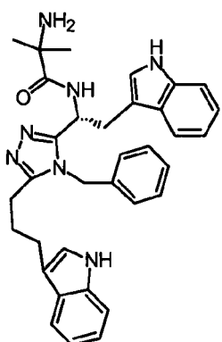
5 compound 10 ( R )- N -(1-(5-(3-(1 H -indol-3-yl)propyl)-4-(3-methoxybenzyl)-4 H -1,2,4-triazol-3-yl)-2-(1 H -indol-3-yl)ethyl)-2-amino-2-methylpropanamide,
