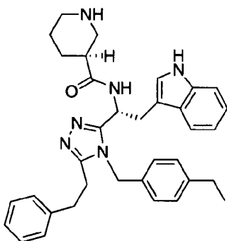
compound 156 N-((R)-1-(4-(4-ethylbenzyl)-5-phenethyl-4H-1,2,4-triazol-3-yl)-2-(1H-indol-3-yl)ethyl)-2-aminobenzamide,
