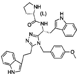
compound 90 (R)-N-((R)-1-(5-(2-(1H-indol-3-yl)ethyl)-4-(4-methoxybenzyl)-4H-1,2,4-triazol-3-yl)-2-(1H-indol-3-yl)ethyl)pyrrolidine-2-carboxamide,
