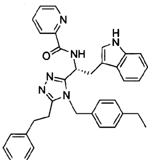
5 compound 139 N-((R)-1-(4-(4-ethylbenzyl)-5-phenethyl-4H-1,2,4-triazol-3-yl)-2-(1H-indol-3-yl)ethyl)-2-aminopyridine-3-carboxamide,
