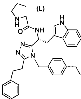
compound 135 N-((R)-1-(4-(4-ethylbenzyl)-5-phenethyl-4H-1,2,4-triazol-3-yl)-2-(1H-indol-3-yl)ethyl)-2-aminoacetamide,
