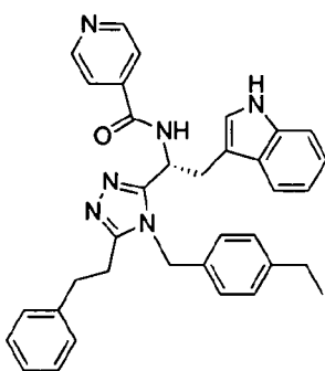
5 compound 142 N-((R)-2-(1H-indol-3-yl)-1-(5-phenethyl-4-phenyl-4H-1,2,4-triazol-3-yl)ethyl)piperidine-4-carboxamide,
