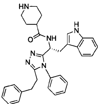
compound 143 (2S)-N-((R)-2-(1H-indol-3-yl)-1-(5-phenethyl-4-phenyl-4H-1,2,4-triazol-3-yl)ethyl)pyrrolidine-2-carboxamide,
