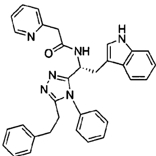
compound 146 N-((R)-2-(1H-indol-3-yl)-1-(5-phenethyl-4-phenyl-4H-1,2,4-triazol-3-yl)ethyl)picolinamide,
