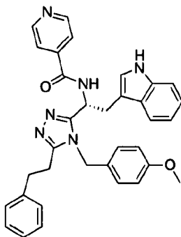
compound 78 ( R )- N -(1-(4-(4-methoxybenzyl)-5-phenethyl-4 H -1,2,4-triazol-3-yl)-2-(1 H -indol-3-yl)ethyl)piperazine-2-carboxamide,
