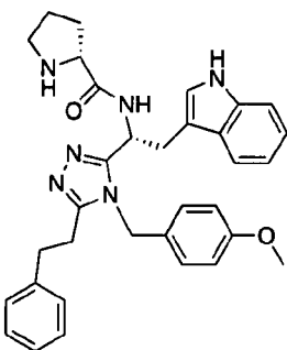
compound 48 (S)-N-((R)-1-(4-(4-methoxybenzyl)-5-phenethyl-4H-1,2,4-triazol-3-yl)-2-(1H-indol-3-yl)ethyl)piperidine-2-carboxamide,
