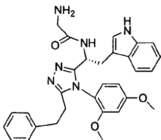
compound 163 N -(( R )-2-(1 H -indol-3-yl)-1-(4-(2,4-dimethoxyphenyl)-5-phenethyl-4 H -1,2,4-triazol-3-yl)ethyl)piperidine-4-carboxamide,
