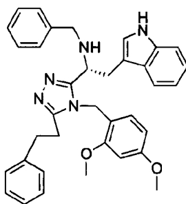
compound 190 (2S)-N-((R)-1-(5-(2-(1H-indol-3-yl)ethyl)-4-(4-methoxybenzyl)-4H-1,2,4-triazol-3-yl)-2-(1H-indol-3-yl)ethyl)-2,5-dihydro-1H-pyrrole-2-carboxamide,
