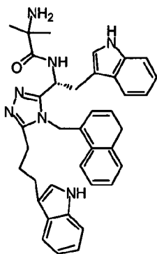
compound 12 ( R )- N -(1-(5-(2-(1 H -indol-3-yl)ethyl)-4-(4-methoxybenzyl)-4 H -1,2,4-triazol-3-yl)-2-(1 H -indol-3-yl)ethyl)-2-amino-2-methylpropanamide,
