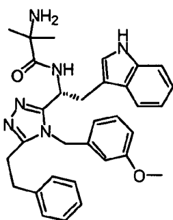
compound 20 (R)-N-(1-(4-(4-methoxybenzyl)-5-phenethyl-4H-1,2,4-triazol-3-yl)-2-(1H-indol-3-yl)ethyl)-2-amino-2-methylpropanamide,
