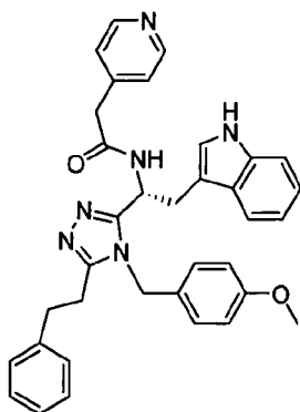
5 compound 53 ( R )- N -(1-(4-(4-methoxybenzyl)-5-phenethyl-4 H -1,2,4-triazol-3-yl)-2-(1 H -indol-3-yl)ethyl)cyclohexanecarboxamide,
