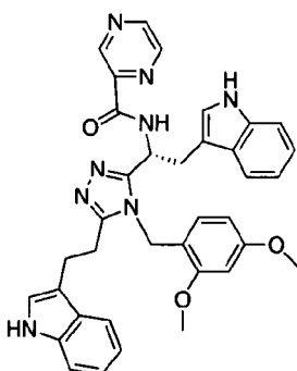
compound 72 (R)-N-1-(5-(2-(1H-indol-3-yl)ethyl)-4-(2,4-dimethoxybenzyl)-4H-1,2,4-triazol-3-yl)-2-(1H-indol-3-yl)ethyl)piperazine-2-carboxamide,
