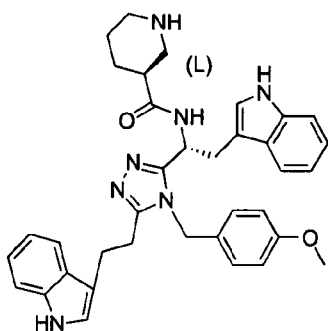
compound 88 (R)-N-((R)-1-(5-(2-(1H-indol-3-yl)ethyl)-4-(4-methoxybenzyl)-4H-1,2,4-triazol-3-yl)-2-(1H-indol-3-yl)ethyl)piperidine-2-carboxamide,
