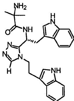
compound 96 ( R )- N -(1-(5-((1 H -indol-3-yl)methyl)-4-methyl-4 H -1,2,4-triazol-3-yl)-2-(1 H -indol-3-yl)ethyl)-2-amino-2-methylpropanamide,
