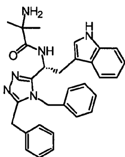
5 compound 110 ( R )- N -(1-(5-benzyl-4-hexyl-4 H -1,2,4-triazol-3-yl)-2-(1 H -indol-3-yl)ethyl)-2-amino-2-methylpropanamide,
