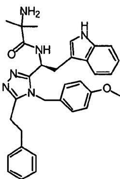
5 compound 130 (R)-N-(1-(4-(4-methoxyphenethyl)-5-phenethyl-4H-1,2,4-triazol-3-yl)-2-(1H-indol-3-yl)ethyl)-2-amino-2-methylpropanamide,
