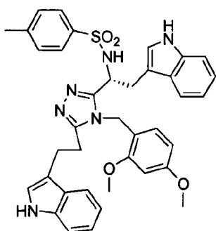
compound 188 N-((R)-1-(4-(2,4-dimethoxybenzyl)-5-phenethyl-4H-1,2,4-triazol-3-yl)-2-(1H-indol-3-yl)ethyl)-4-azidobenzamide,
