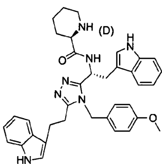
5 compound 89 (S)-N-((R)-1-(5-(2-(1H-indol-3-yl)ethyl)-4-(4-methoxybenzyl)-4H-1,2,4-triazol-3-yl)-2-(1H-indol-3-yl)ethyl)pyrrolidine-2-carboxamide,
