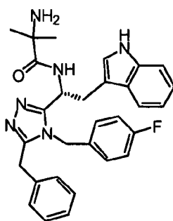
5 compound 31 ( R )- N -(1-(5-(2-(1 H -indol-3-yl)ethyl)-4-(2,4-dimethoxybenzyl)-4 H -1,2,4-triazol-3-yl)-2-(1 H -indol-3-yl)ethyl)piperidine-4-carboxamide,
