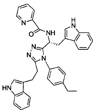
5 compound 148 N-((R)-1-(5-(2-(1H-indol-3-yl)ethyl)-4-(4-ethylphenyl)-4H-1,2,4-triazol-3-yl)-2-(1H-indol-3-yl)ethyl)-2-(pyridin-2-yl)acetamide,
