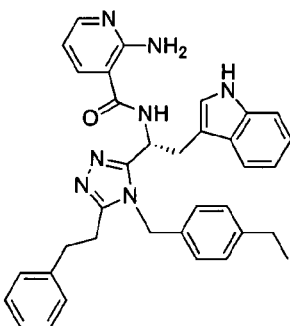
compound 140 (2S)-N-((R)-1-(4-(4-ethylbenzyl)-5-phenethyl-4H-1,2,4-triazol-3-yl)-2-(1H-indol-3-yl)ethyl)-2-aminopropanamide,
