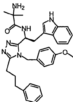
5 compound 126 (S)-N-(1-(4-(4-methoxybenzyl)-5-benzyl-4H-1,2,4-triazol-3-yl)-2-(1H-indol-3-yl)ethyl)-2-amino-2-methylpropanamide,
