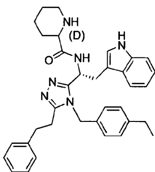
compound 138 N-((R)-1-(4-(4-ethylbenzyl)-5-phenethyl-4H-1,2,4-triazol-3-yl)-2-(1H-indol-3-yl)ethyl)picolinamide,
