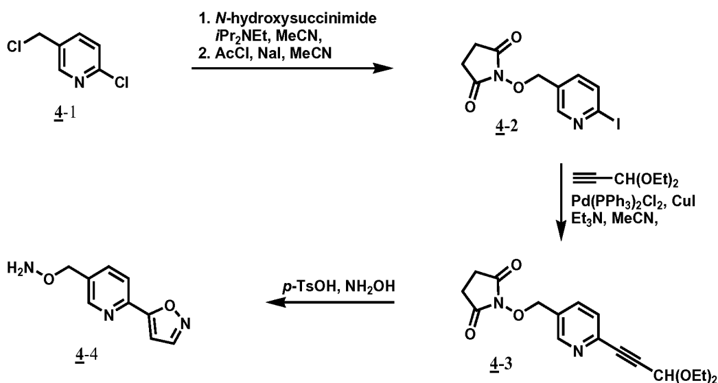
Scheme 4
