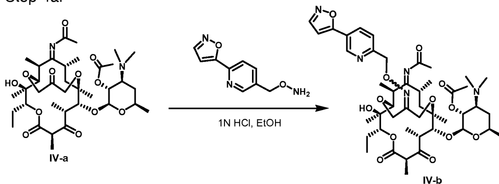
Compound 4
