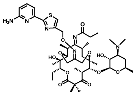
Compound 3
