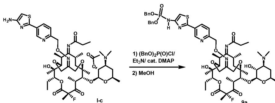
Compound 9
