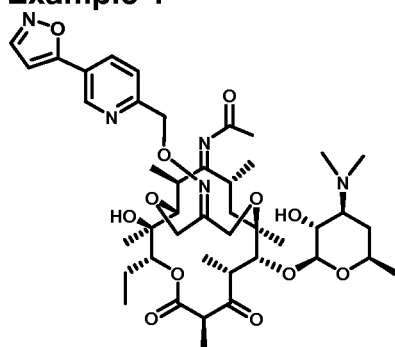
Compound 4
