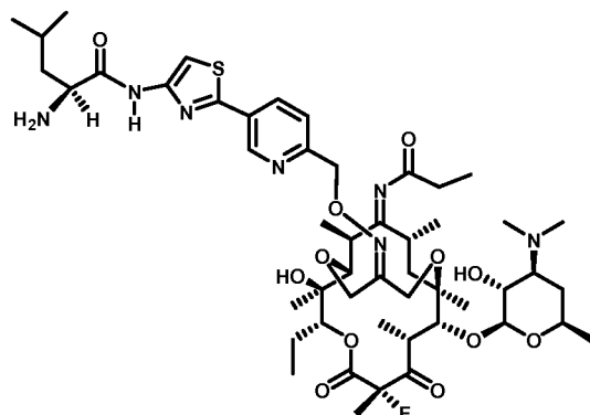
Compound 6
