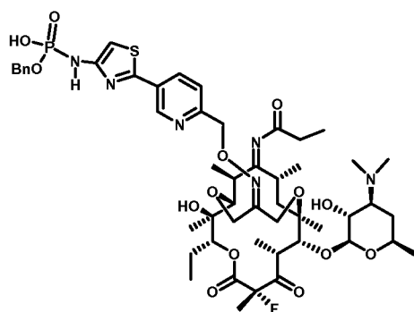
Compound 9
