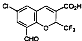
6-Chloro-8-Formyl-2-(trifluoromethyl)-2H-1-benzopyran-3-carboxylic acid
