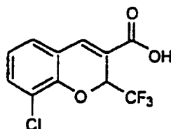
8-Chloro-2-trifluoromethyl-2H-1-benzopyran-3-carboxylic acid
