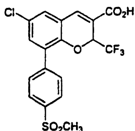
6-Chloro-8-[(4-methylsulfonyl)phenyl]-2-(trifluoromethyl)-2H-1-benzopyran-3-carboxylic acid
