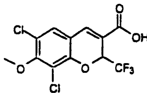
6,8-Dichloro-7-methoxy-2-trifluoromethyl-2H-1-benzopyran-3-carboxylic acid
