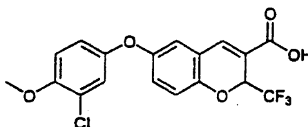
6-(3-Chloro-4-methoxyphenoxy)-2-(trifluoromethyl)-2H-1-benzopyran-3-carboxylic acid
