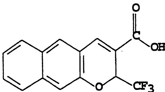
2-Trifluoromethyl-2H-naphtho[2,3-b]pyran-3-carboxylic acid
