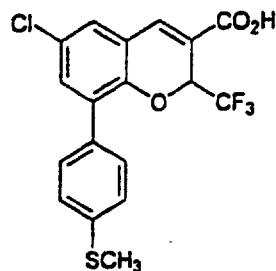
6-Chloro-8-[(4-methylthio)phenyl]-2-(trifluoromethyl)-2H-1-benzopyran-3-carboxylic acid
