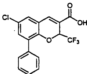
6-Chloro-8-phenyl-2-(trifluoromethyl)-2H-1-benzopyran-3-carboxylic acid
