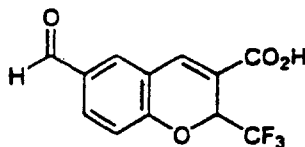
6-Formyl-2-(trifluoromethyl)-2H-1-benzopyran-3-carboxylic acid
