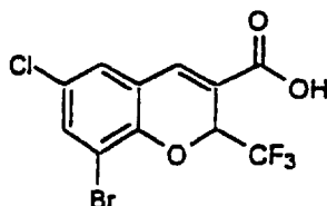
8-Bromo-6-chloro-2-trifluoromethyl-2H-1-benzopyran-3-carboxylic acid
