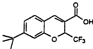
25 7-(1,1-Dimethylethyl)-2-trifluoromethyl-2H-1-benzopyran-3-carboxylic acid
