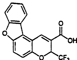
3-(Trifluoromethyl)-3H-benzofuro[3,2-f][1]benzopyran-2-carboxylic acid
