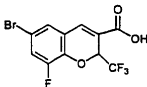
6-Bromo-8-fluoro-2-(trifluoromethyl)-2H-1-benzopyran-3-carboxylic acid
