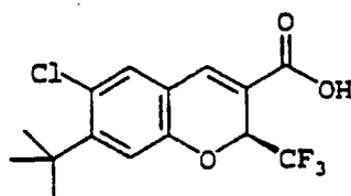
(S)-6-Chloro-7-(1,1-dimethylethyl)-2-(trifluoromethyl)-2H-1-benzopyran-3-carboxylic acid
