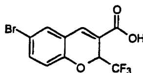
6-Bromo-2-trifluoromethyl-2H-1-benzopyran-3-carboxylic acid
