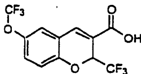
6-Trifluoromethoxy-2-trifluoromethyl-2H-1-benzopyran-3-carboxylic acid
