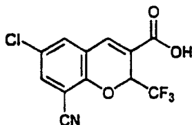
6-Chloro-8-cyano-2-(trifluoromethyl)-2H-1-benzopyran-3-carboxylic acid
