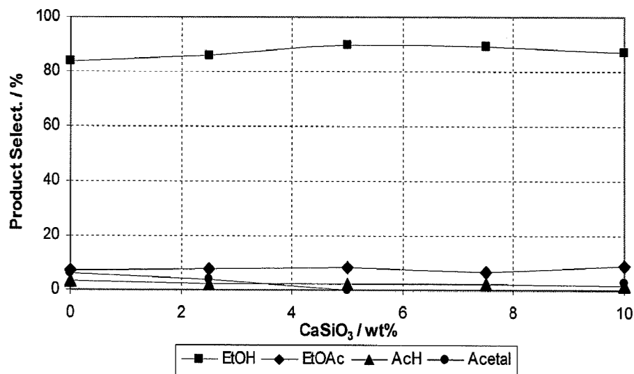
FIG. 6C - Selectivity @ 250
