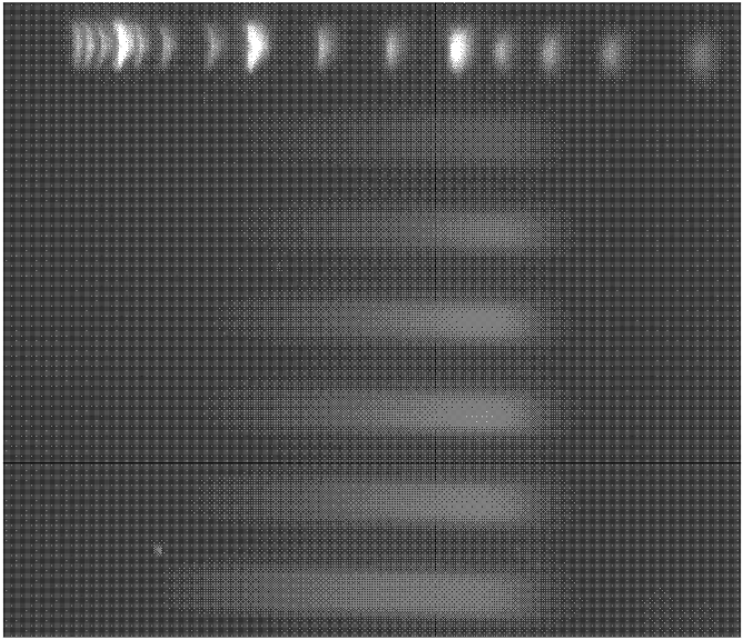
Two rounds of Nick-ligate With Segmentase
