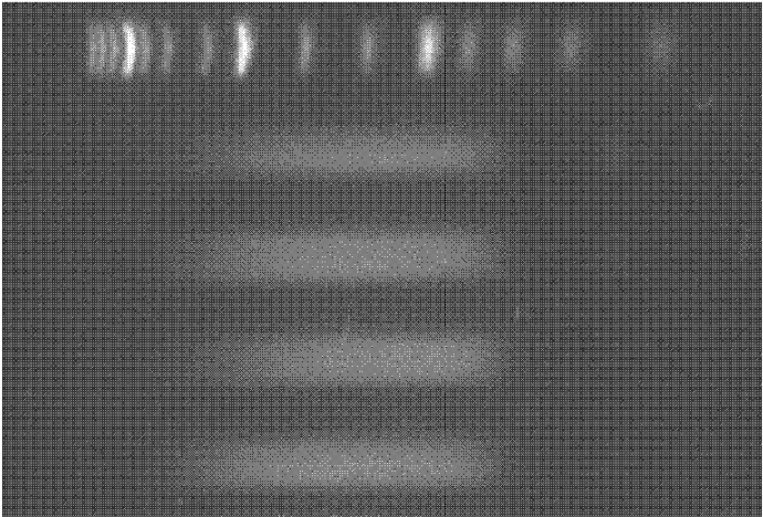
Two rounds of Nick-ligate With masterase
