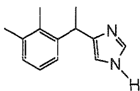
Medetomidine
