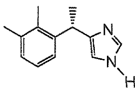
Dexmedetomidine
