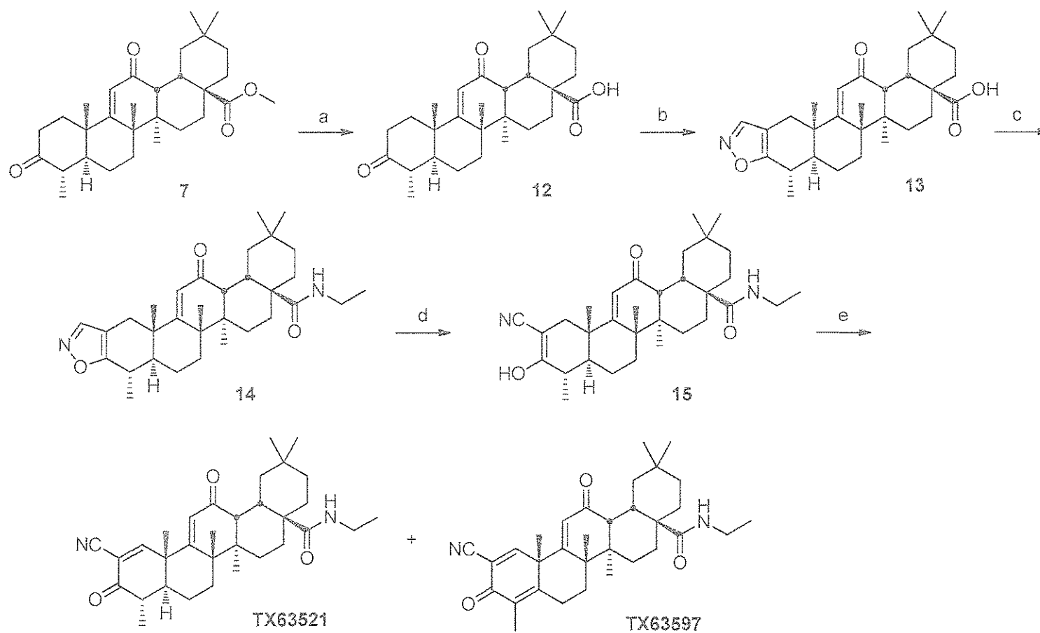
Scheme 4. Alternative synthetic route to TX63521
