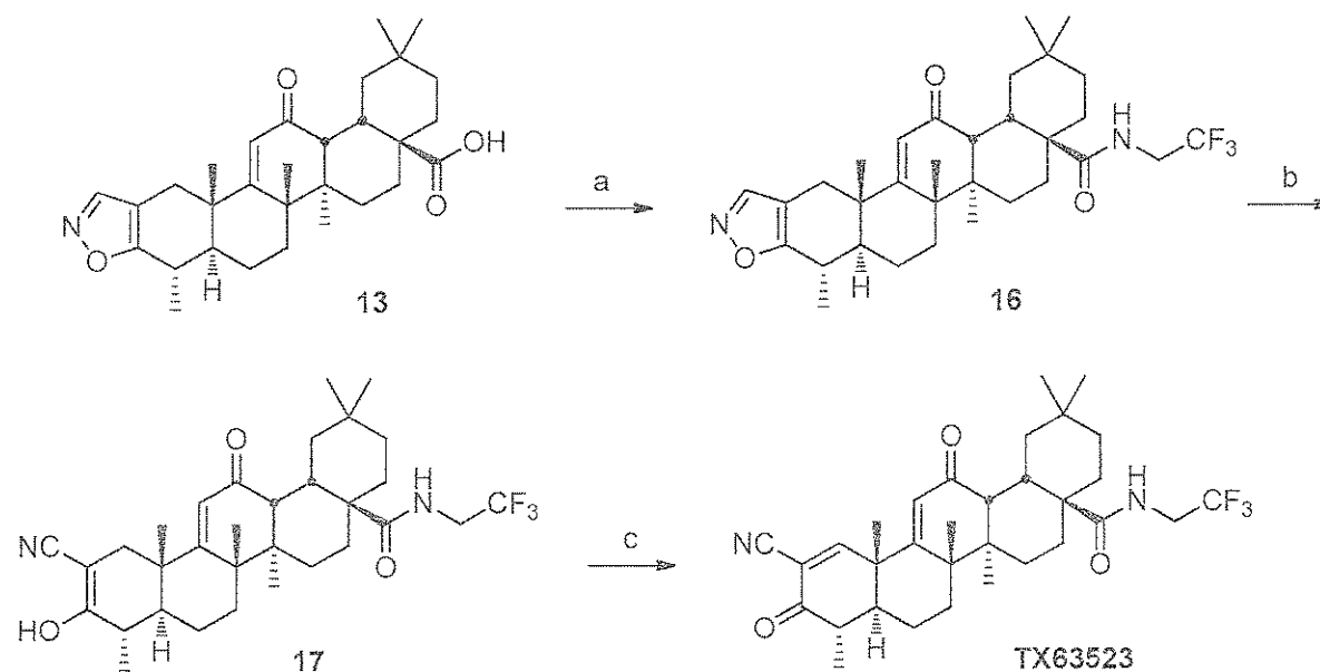
Scheme 7. Alternative synthetic route to TX63523
