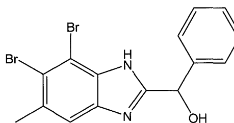
Compound 16
