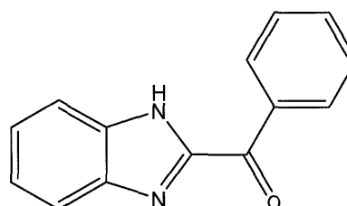
Compound 12
