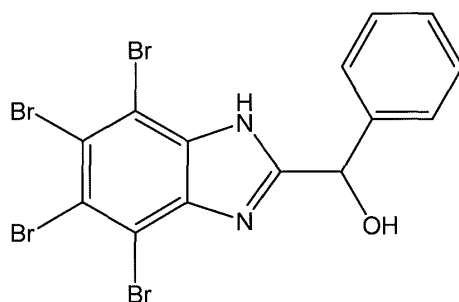
Compound 20
