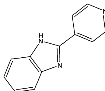
Compound 6
