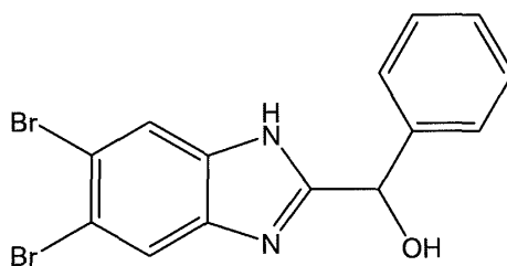
Compound 18
