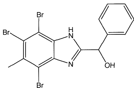
Compound 17
