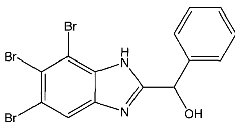
Compound 19
