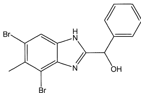
Compound 15
