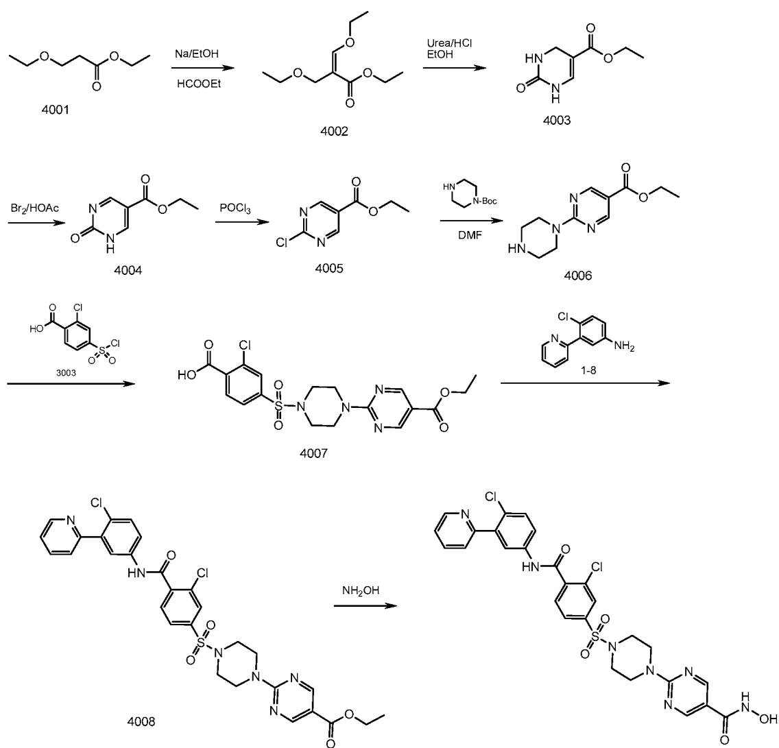
Scheme 4
