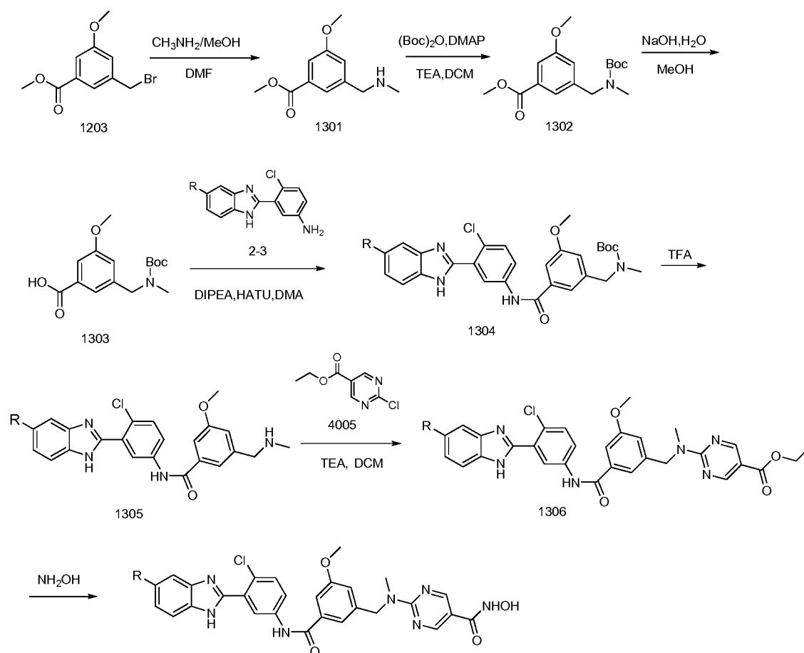
Scheme 13
