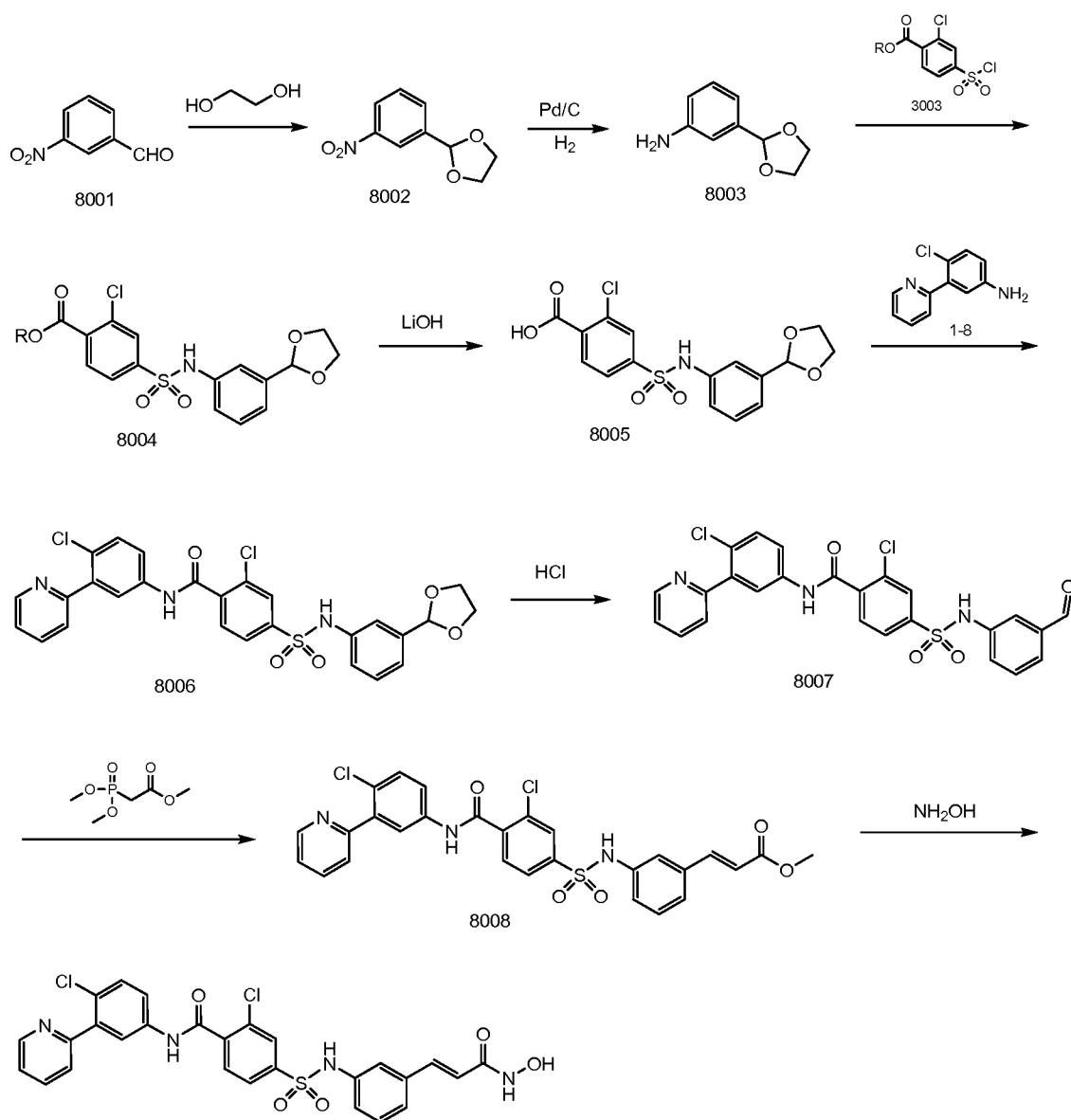
Scheme 8
