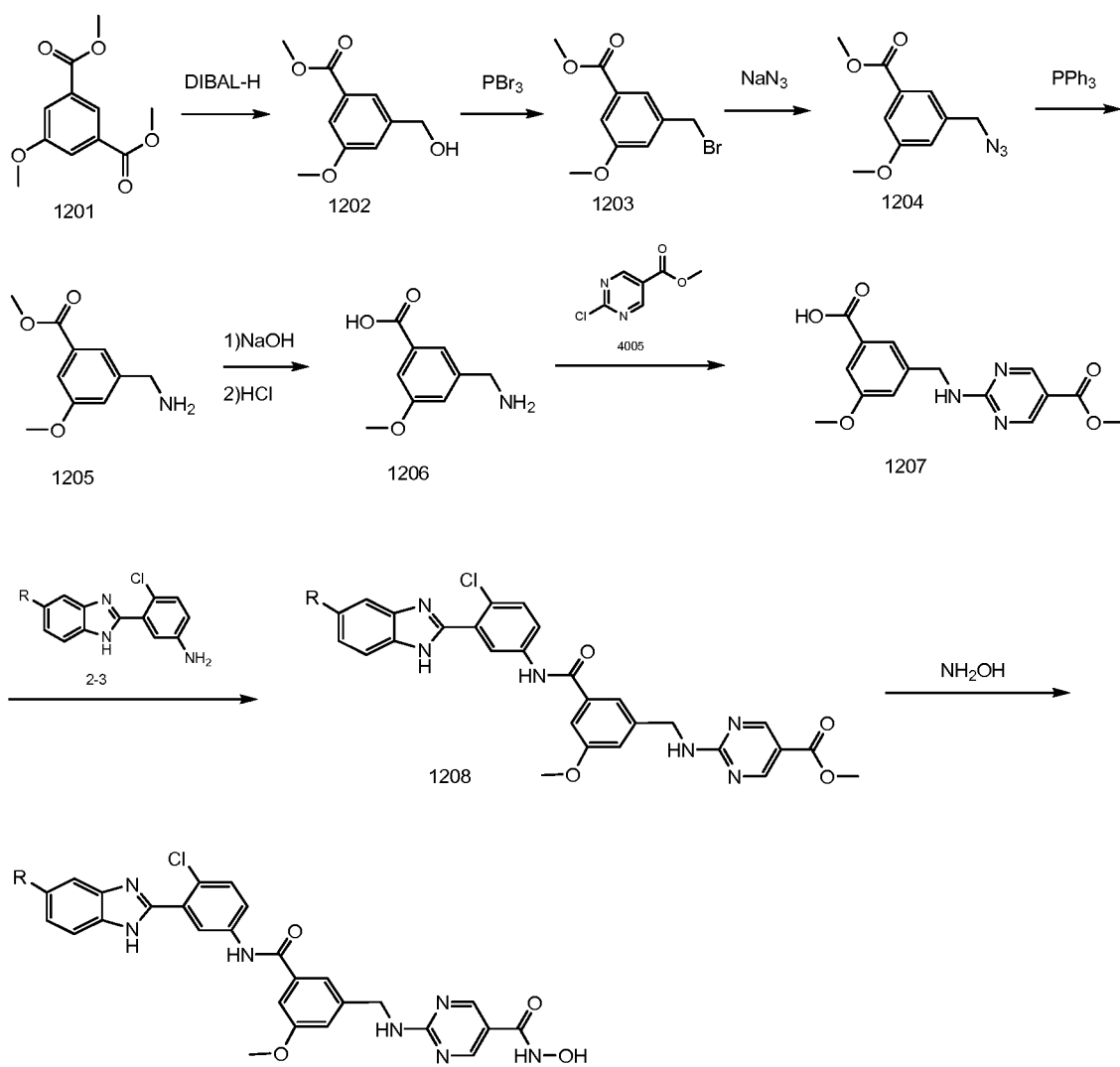
Scheme 12
