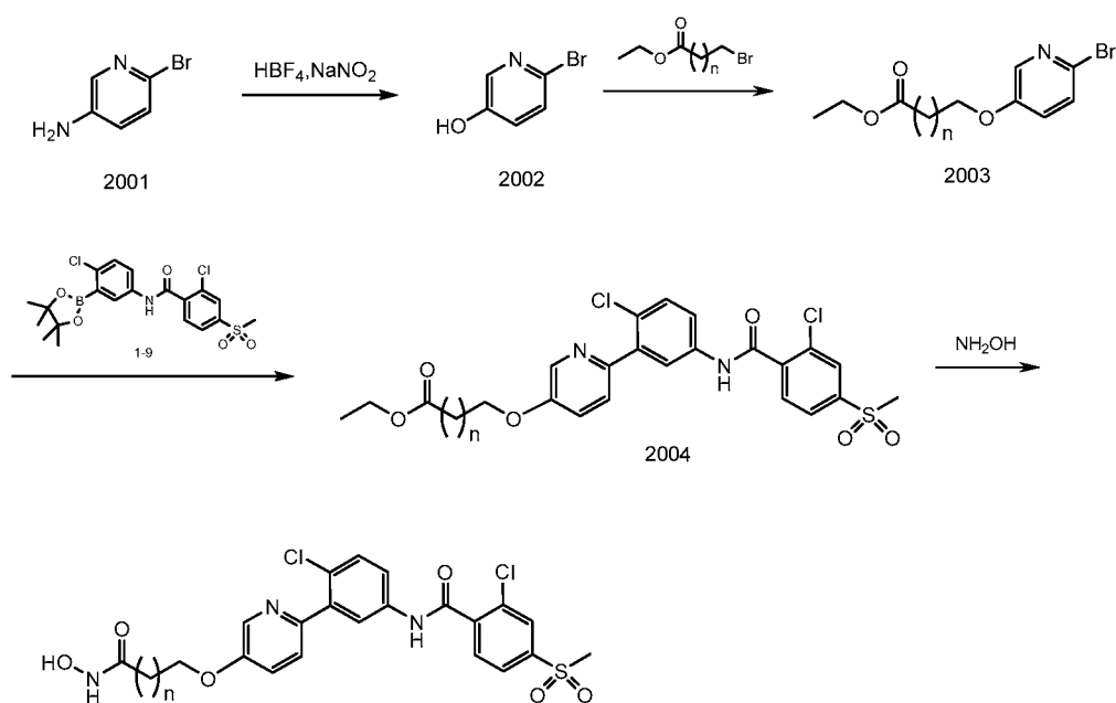
Scheme 2
