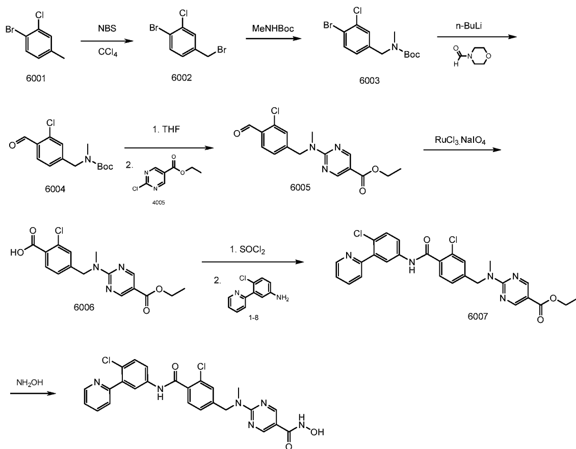
Scheme 6
