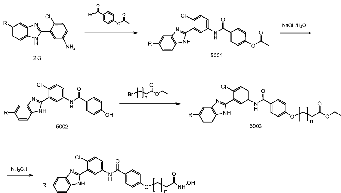
Scheme 6
