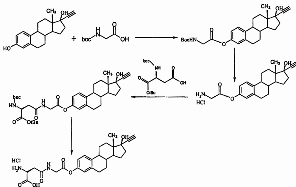
Reaction Sequence 10
