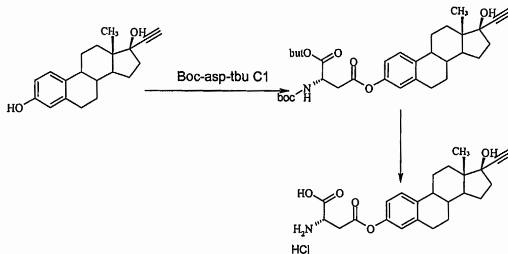
Reaction Sequence 12
