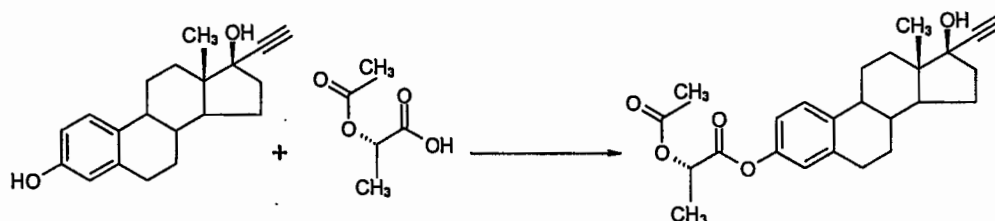
Reaction Sequence 8
