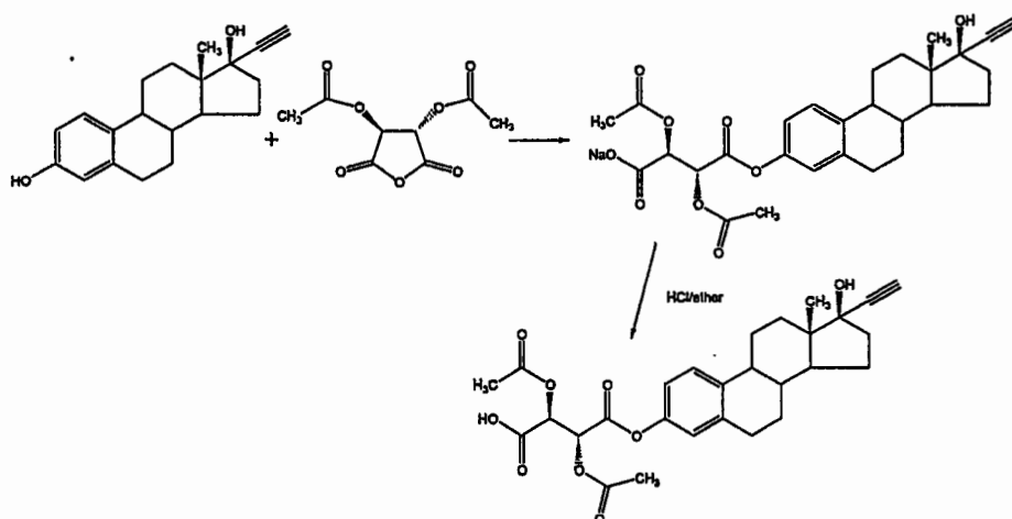
Reaction Sequence 9
