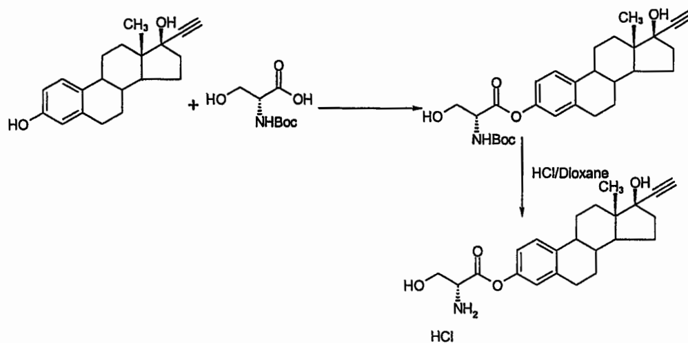
Reaction Sequence 7
