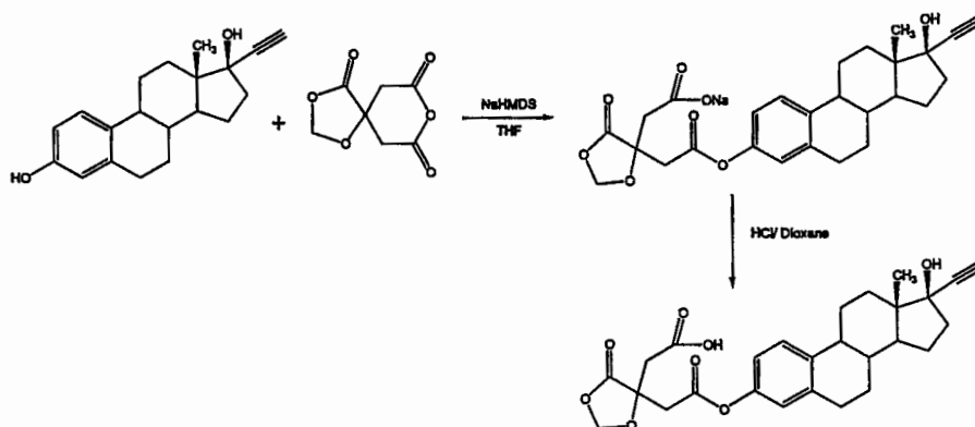
Reaction Sequence 2
