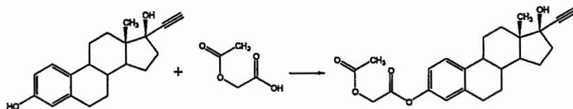
Reaction Sequence 5
