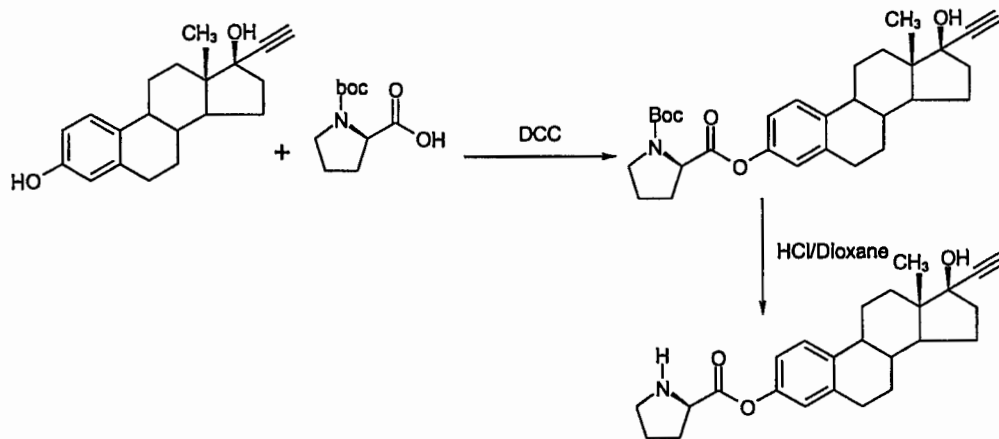
Reaction Sequence 6
