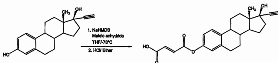
Reaction Sequence 1
