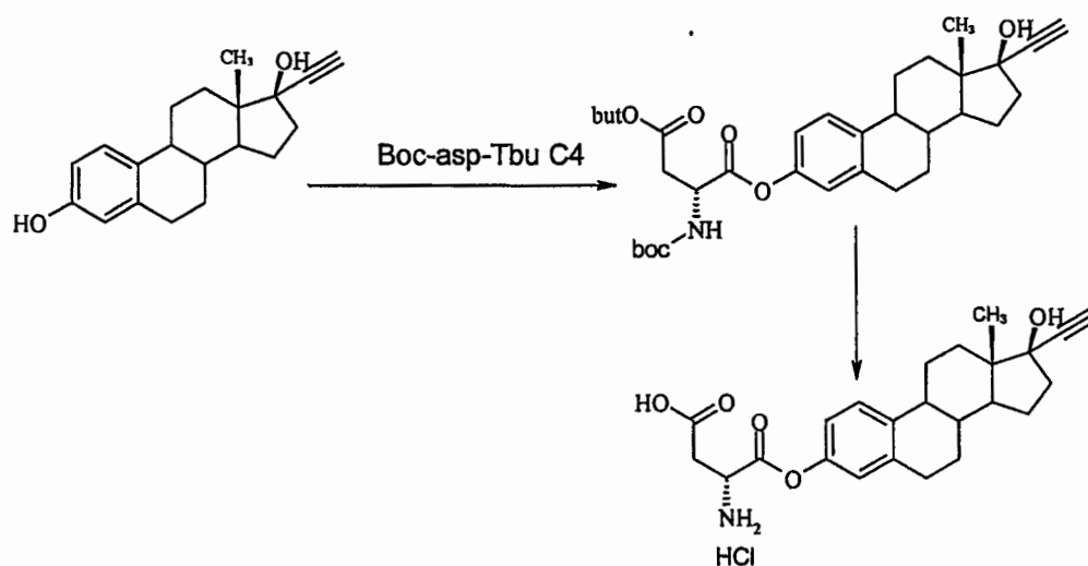
Reaction Sequence 11
