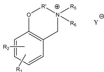
(Formula Ib)
