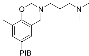
(Compound 4)
