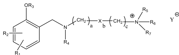
(Formula Ia)
