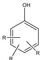
(Formula II)
