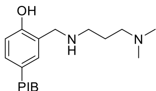
(Compound 11)
