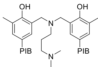
(Compound 9)
