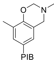
(Compound 8)
