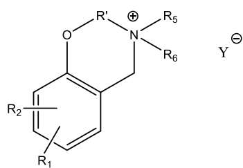
(Formula Ib)
