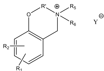
(Formula Ib)
