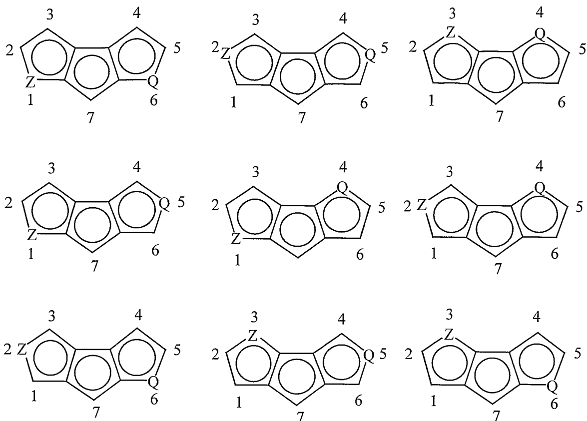
heterofluorenyl ligands
