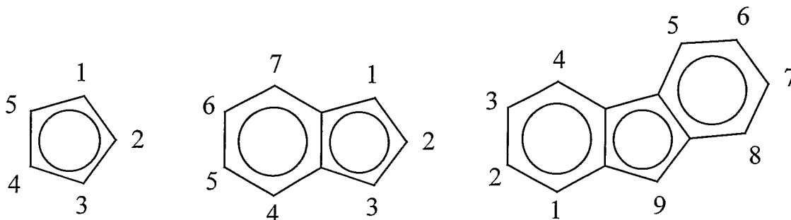
Cyclopentadienyl
