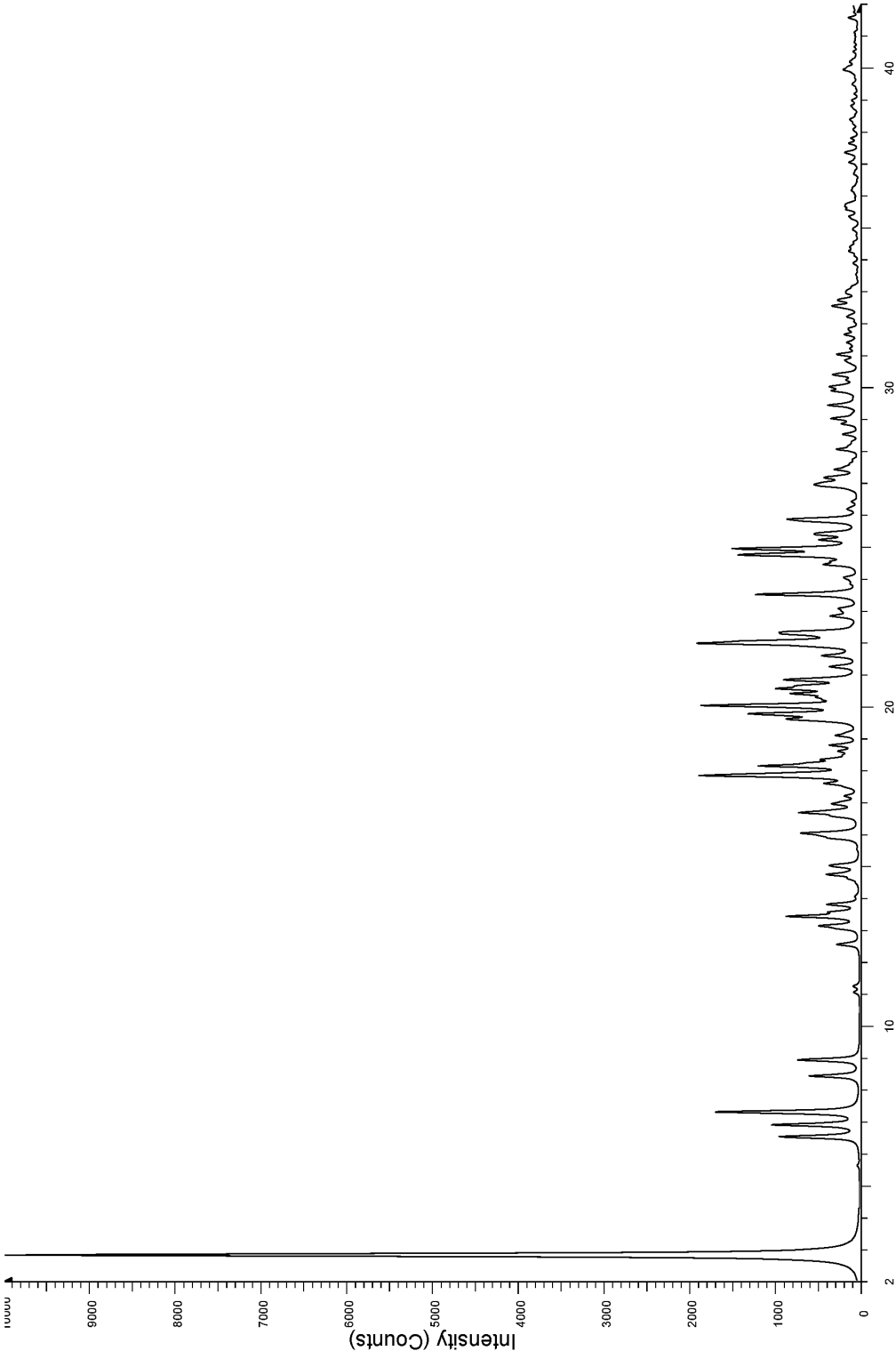
2 Theta Angle
