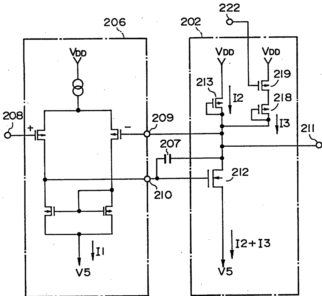
n - TYPE OP-AMP PROVIDED WITH CURRENT-CONTROL FUNCTION
