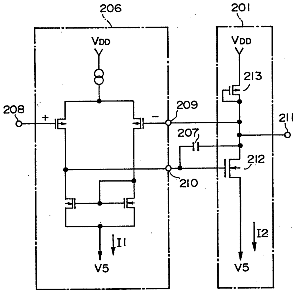
n-TYPE OP-AMP
