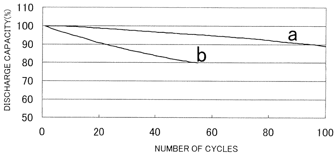
FIG. 2 CYCLE TEST AT 60° C
