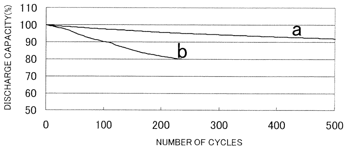
FIG. 1 CYCLE TEST AT 25° C
