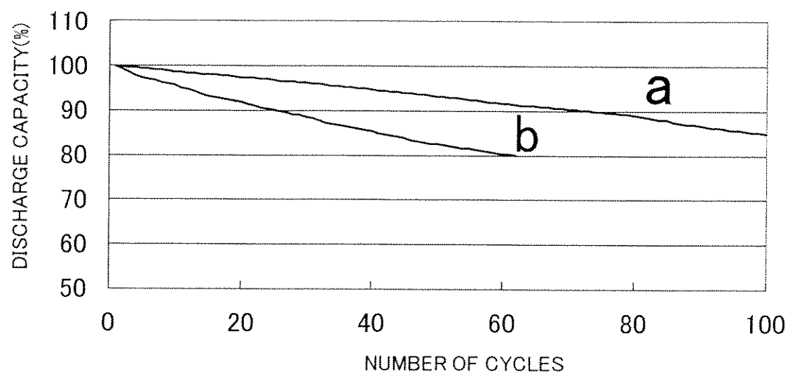
FIG. 3 CYCLE TEST AT -10^{\circ} C
