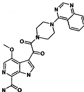
4-methoxy-3-(2-oxo-2-(4-(quinazolin-4-yl)piperazin-1-yl)acetyl)-1H-pyrrolo[2,3-c]pyridine-7-carboxamide
