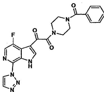
Compound IVb
