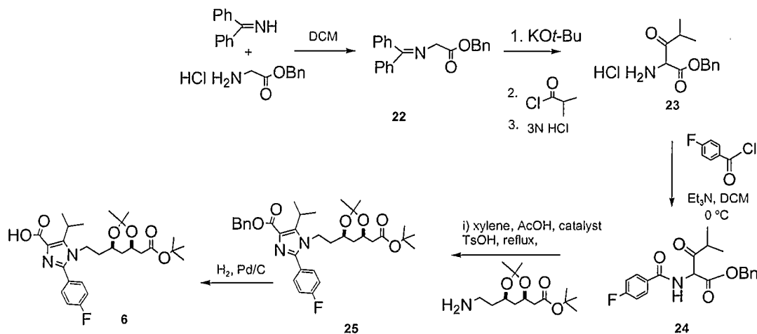
Scheme 7
