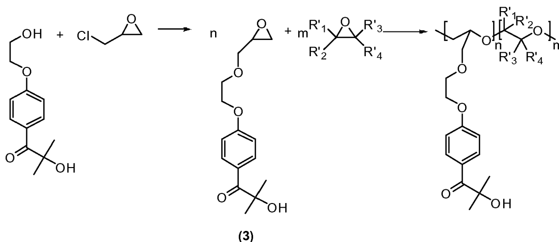
Scheme 3: Preparation of polymeric photoinitiator from Irgacure 2959.
