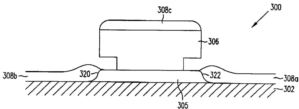
FIG. 3c (Prior Art)
