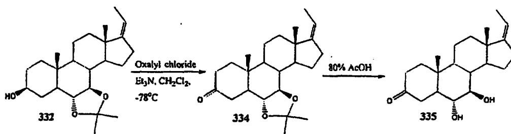
Scheme 81
