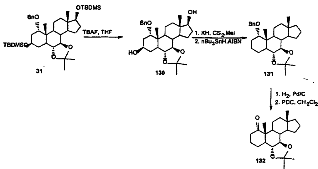
Scheme 41
