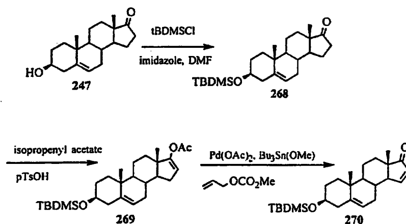
Scheme 66
