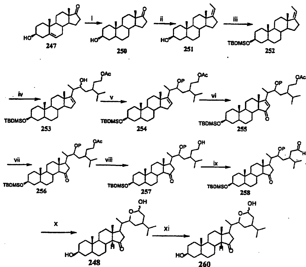
Scheme 64
