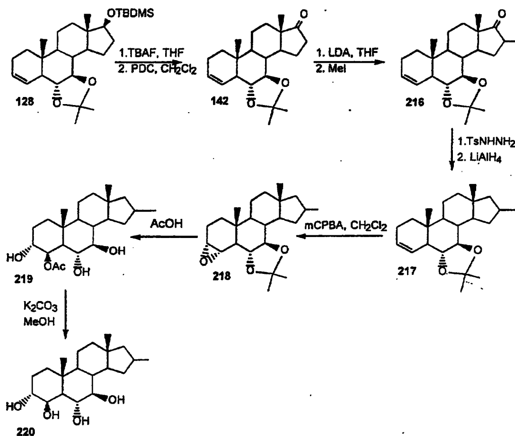
Scheme 52
