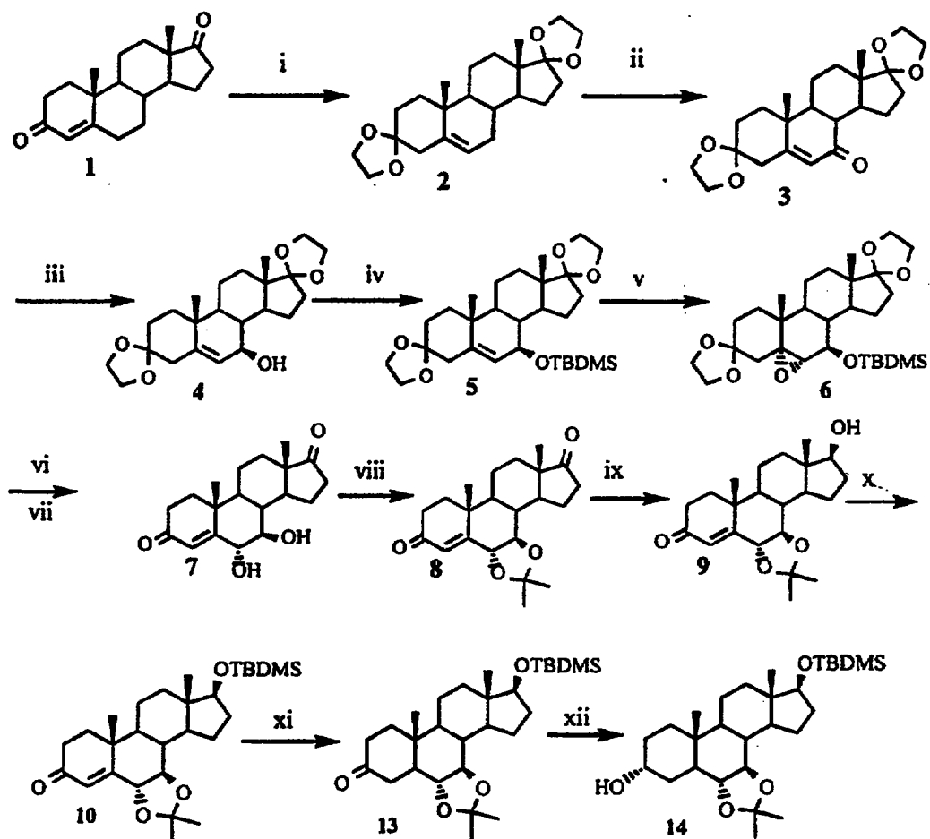
Scheme 79
