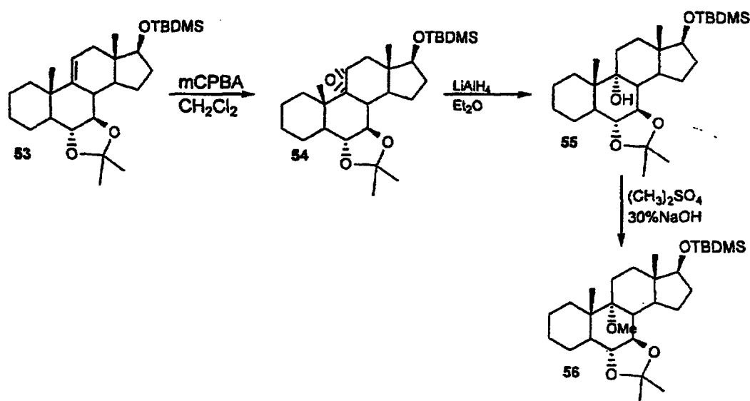
Scheme 17
