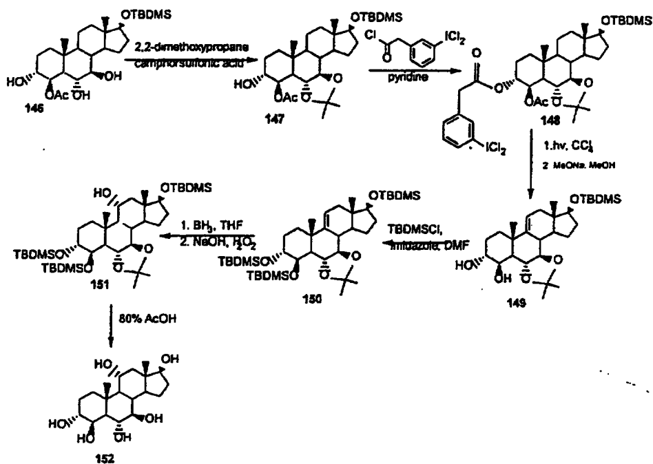
Scheme 44
