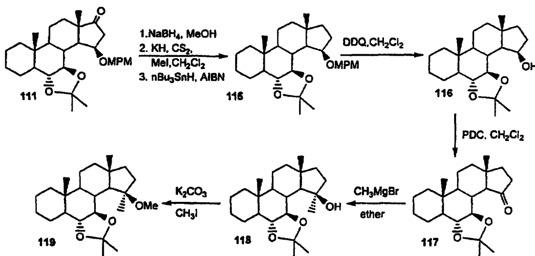
Scheme 34
