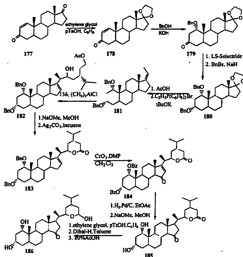
Scheme 48
