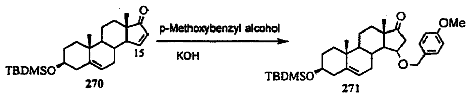
Scheme 67
