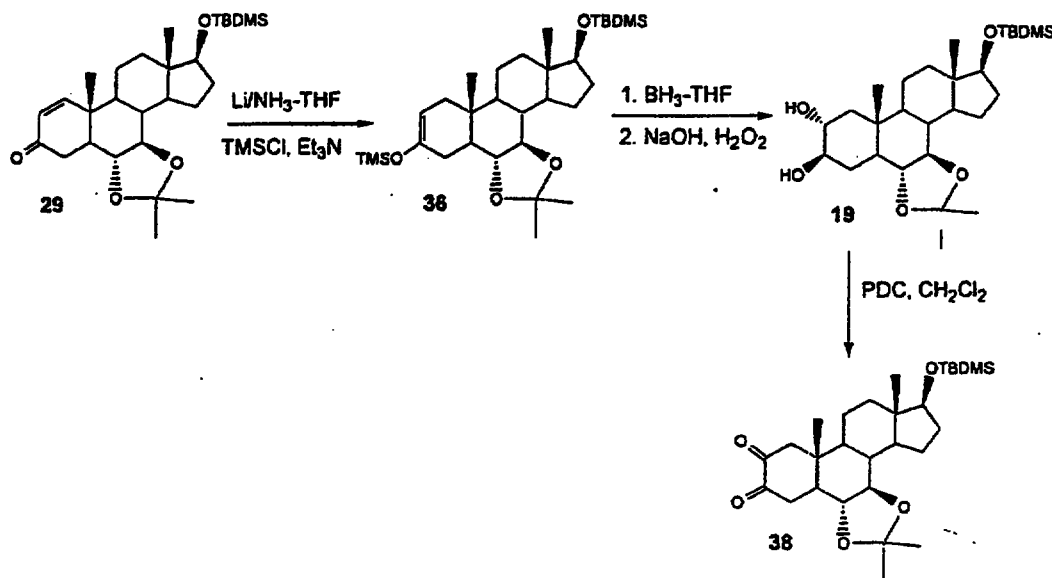
Scheme 9
