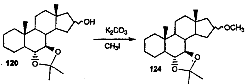
Scheme 36
