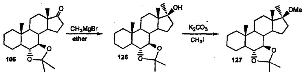
Scheme 38
