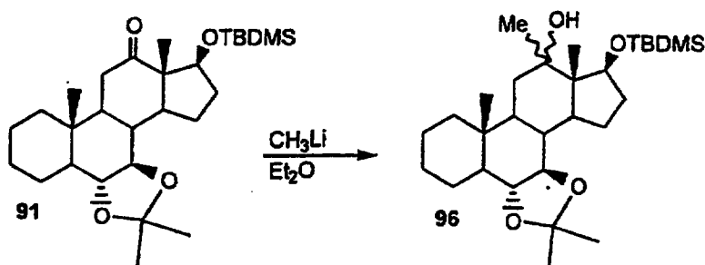
Scheme 28
