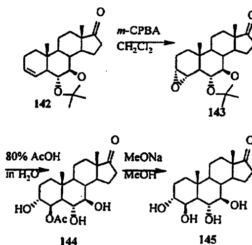
Scheme 43
