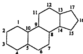
Structure 1
