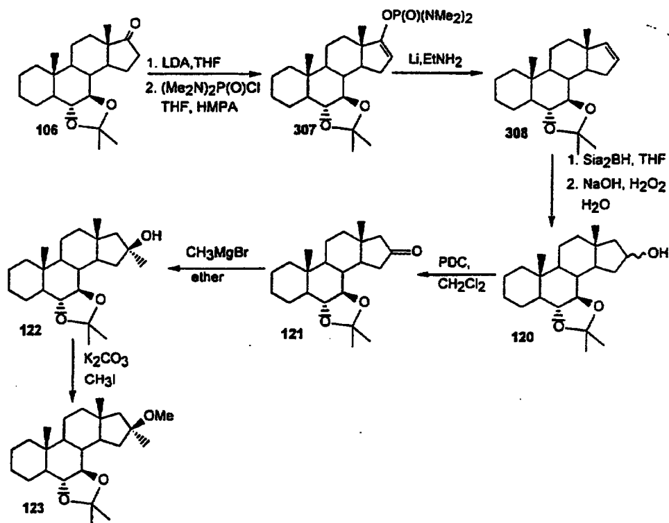
Scheme 35
