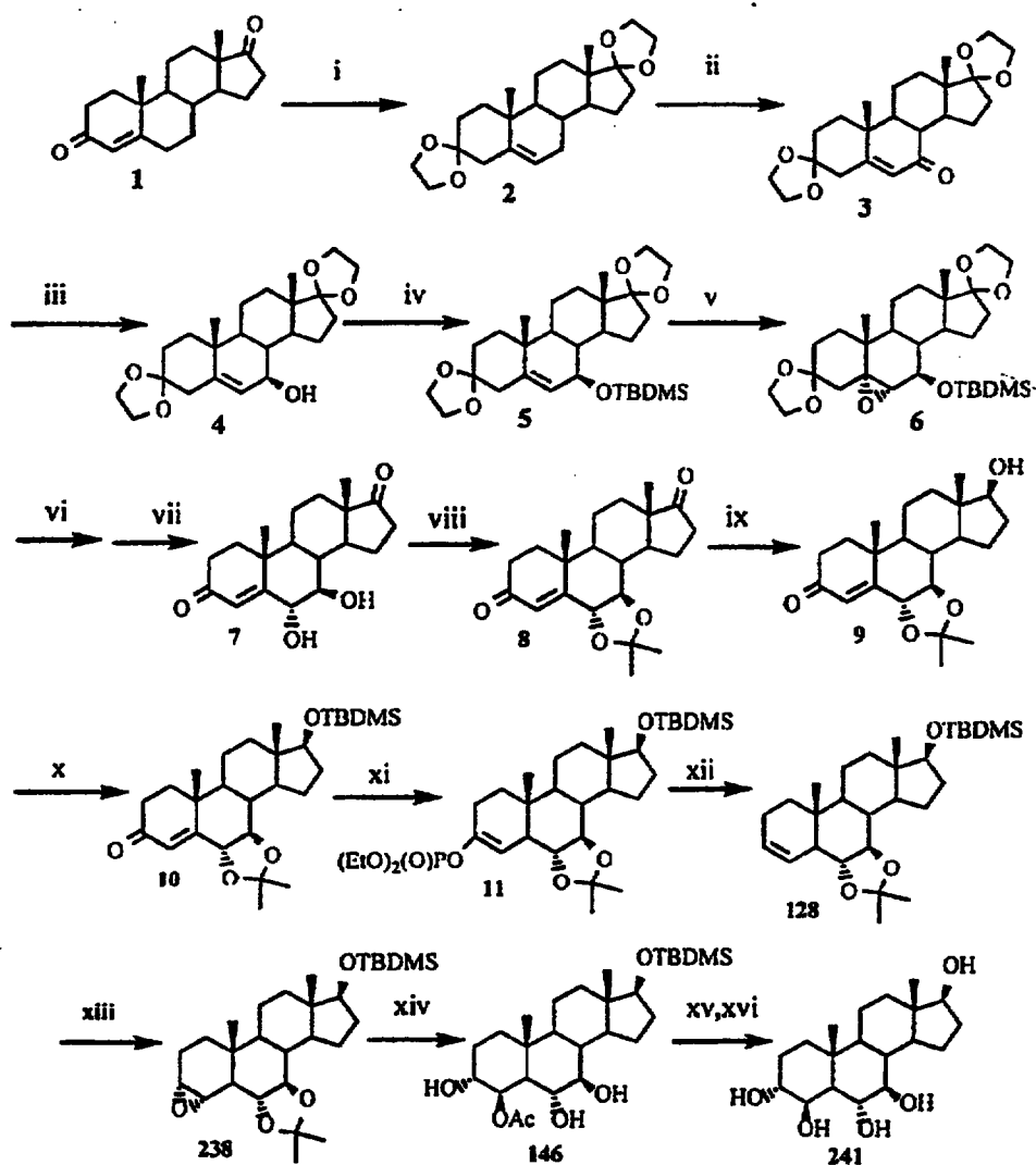
Scheme 61
