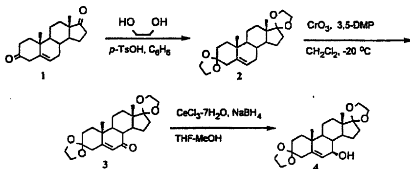
Scheme 56
