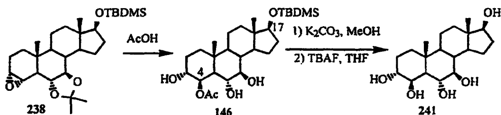
Scheme 62
