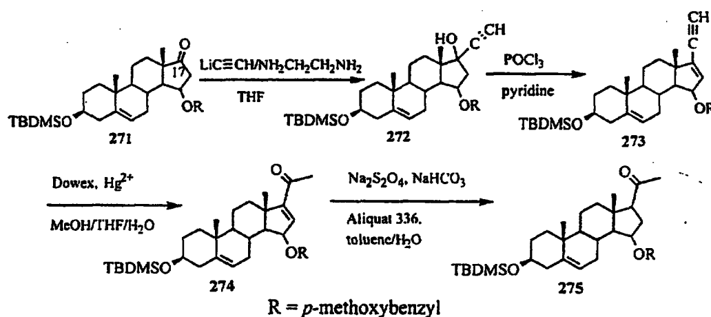
Scheme 68
