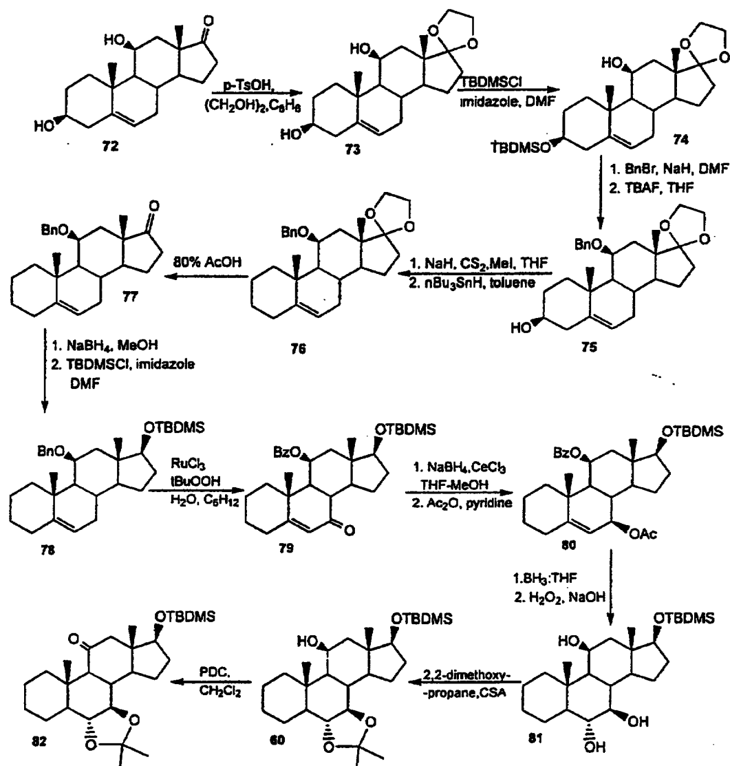
Scheme 22
