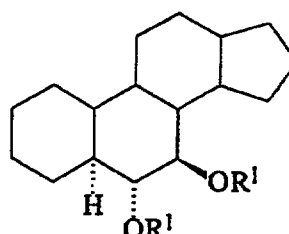
Structure 4
