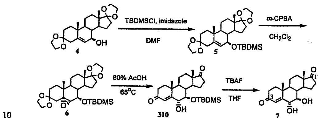
Scheme 57
