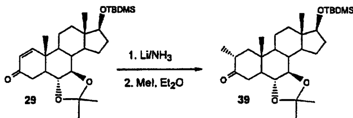
Scheme 10
