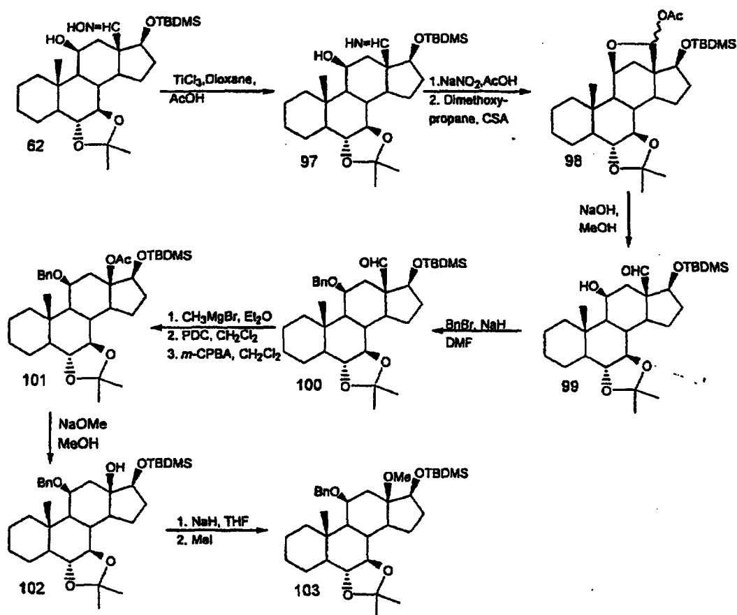
Scheme 29
