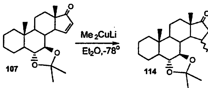
Scheme 33
