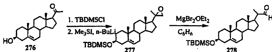
Scheme 69
