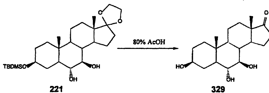
Scheme 78
