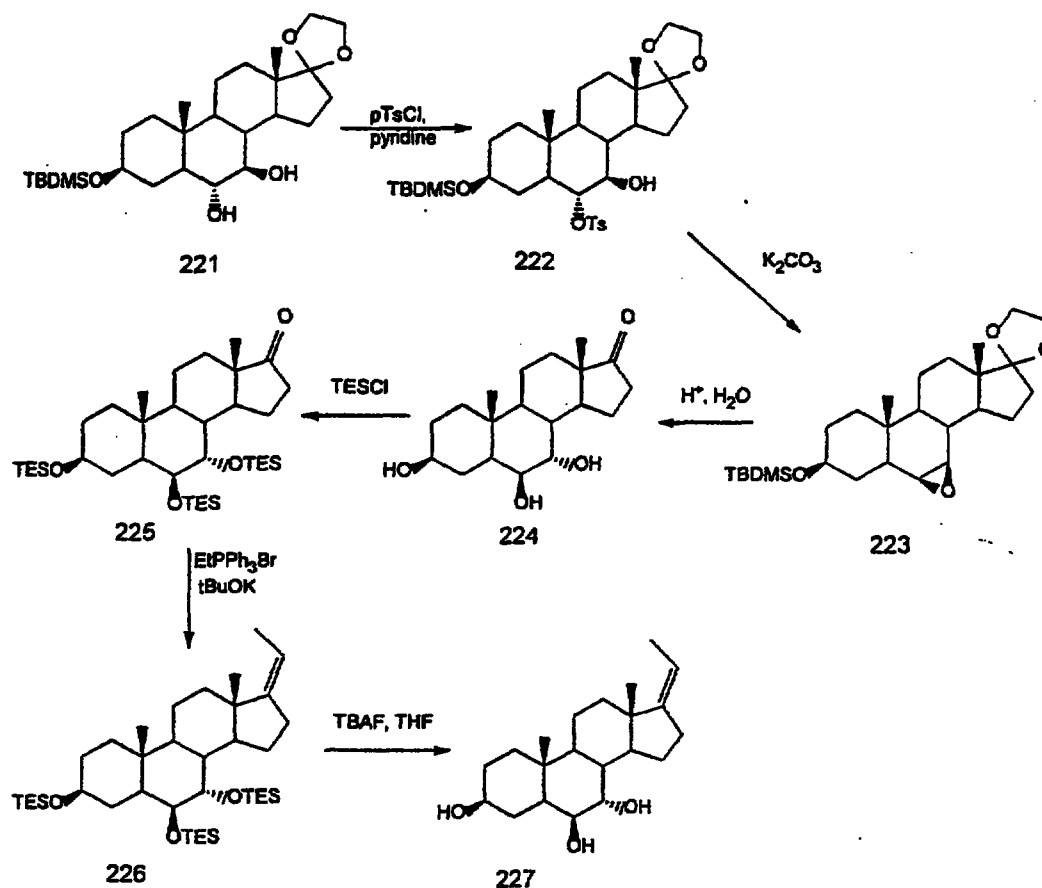
Scheme 53
