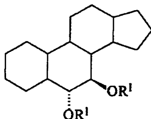
Structure 3
