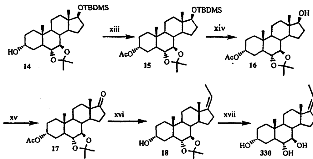
Scheme 79 (continued).
