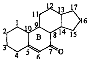
Formula (13)
