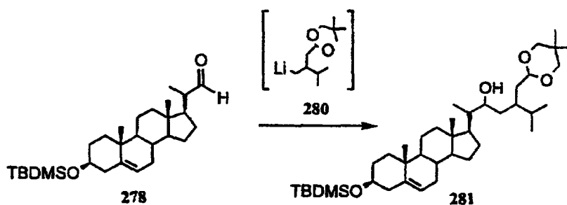
Scheme 70
