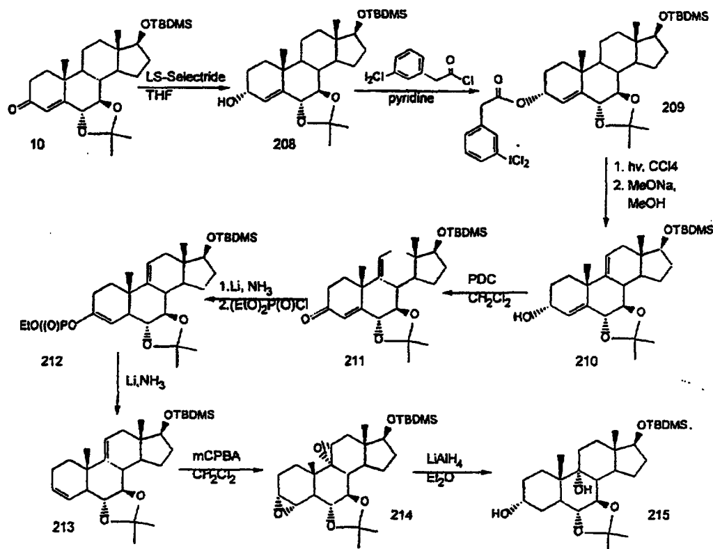
Scheme 51
