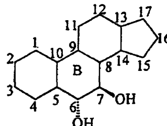
Formula (14)
