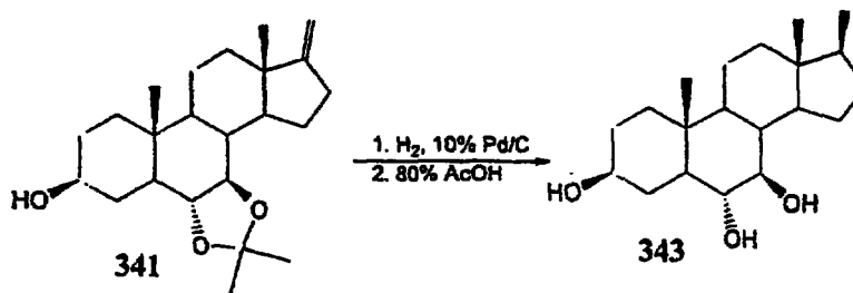
Scheme 87
