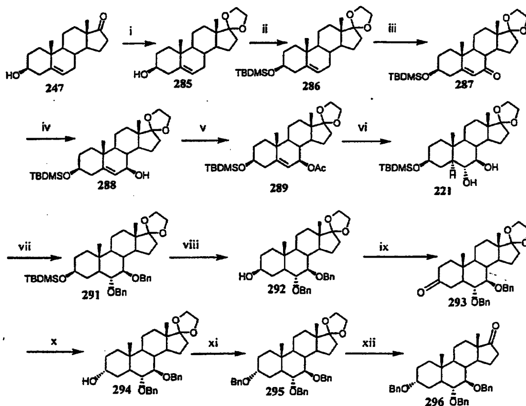
Scheme 73
