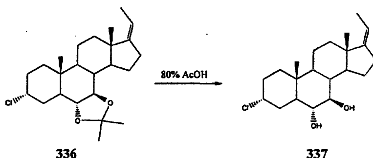
Scheme 82
