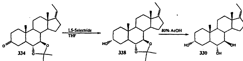
Scheme 83
