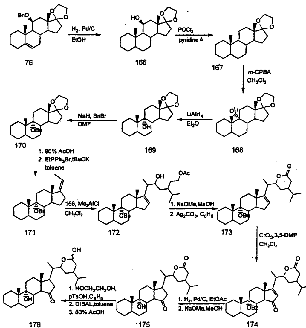
Scheme 47
