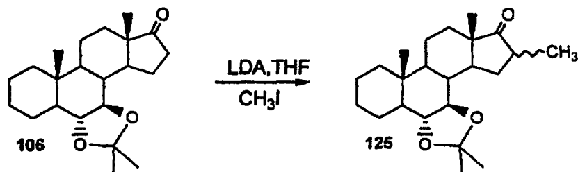
Scheme 37
