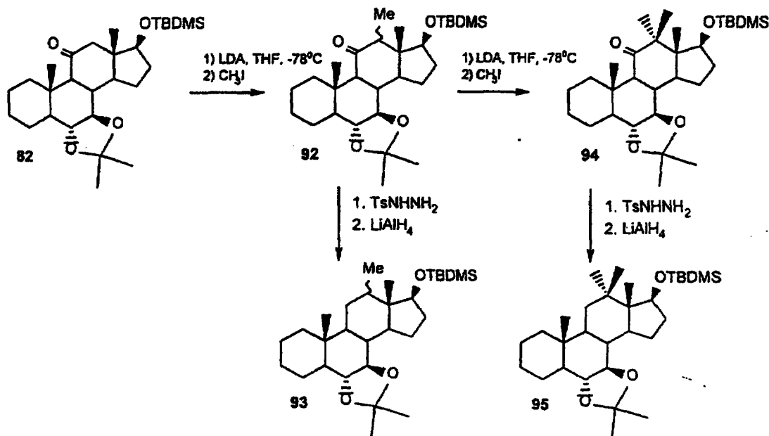
Scheme 27
