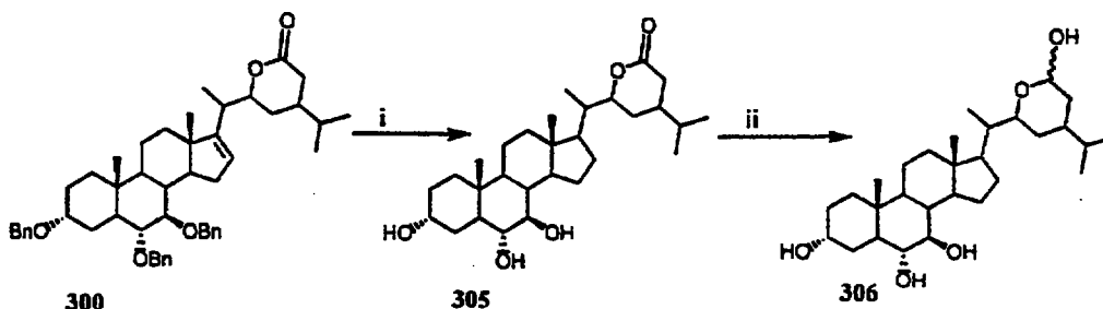
Scheme 74
