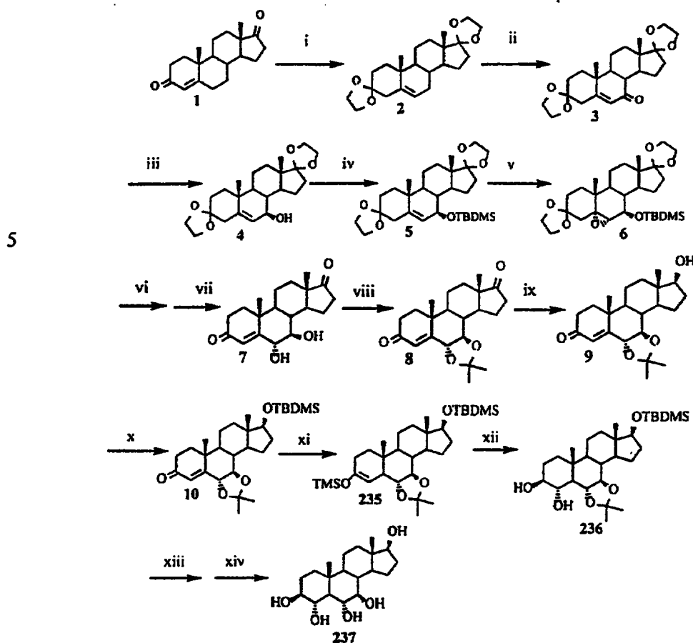
Scheme 55
