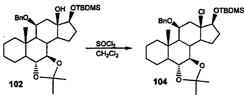
Scheme 30
