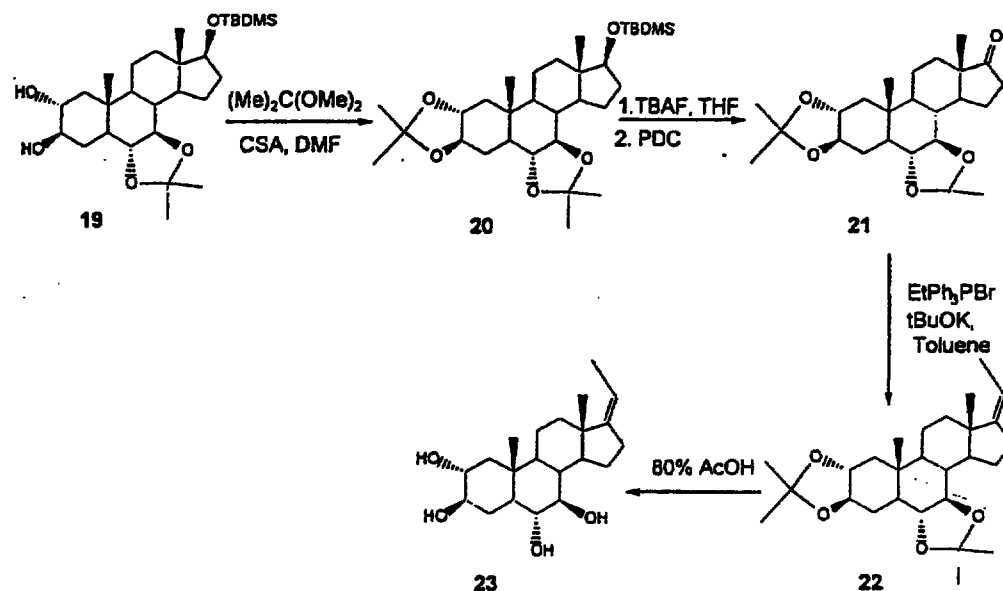
Scheme 4
