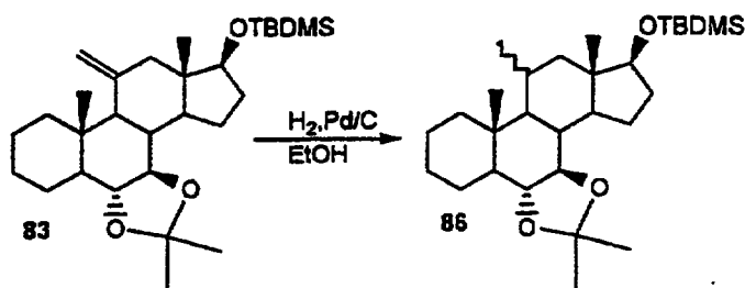
Scheme 24
