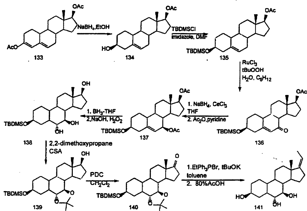
Scheme 42
