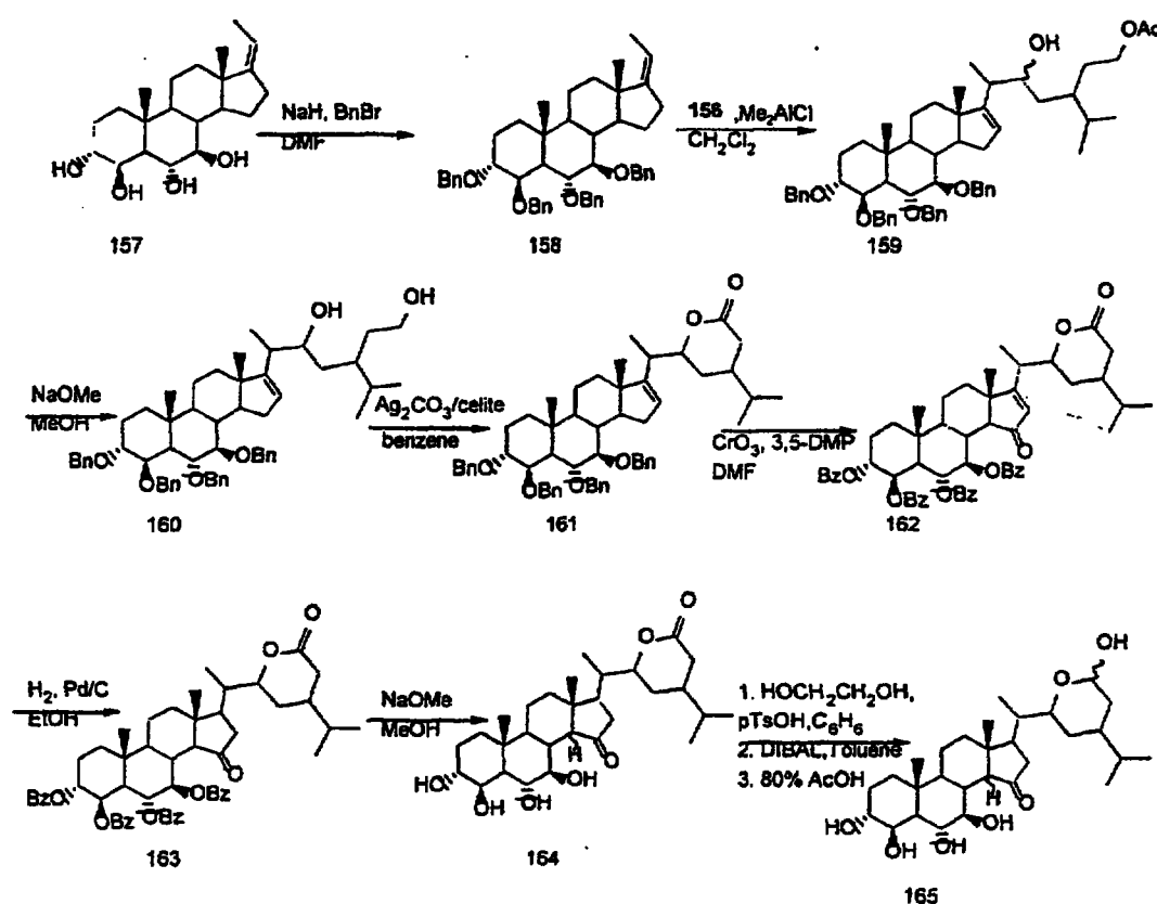
Scheme 46
