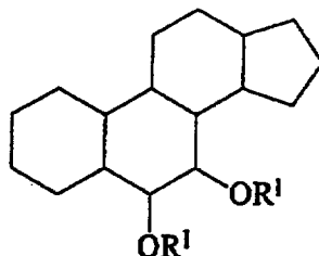
Structure 2
