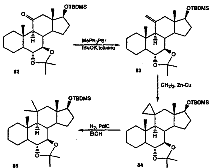
Scheme 23
