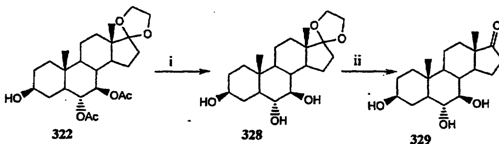
Scheme 77
