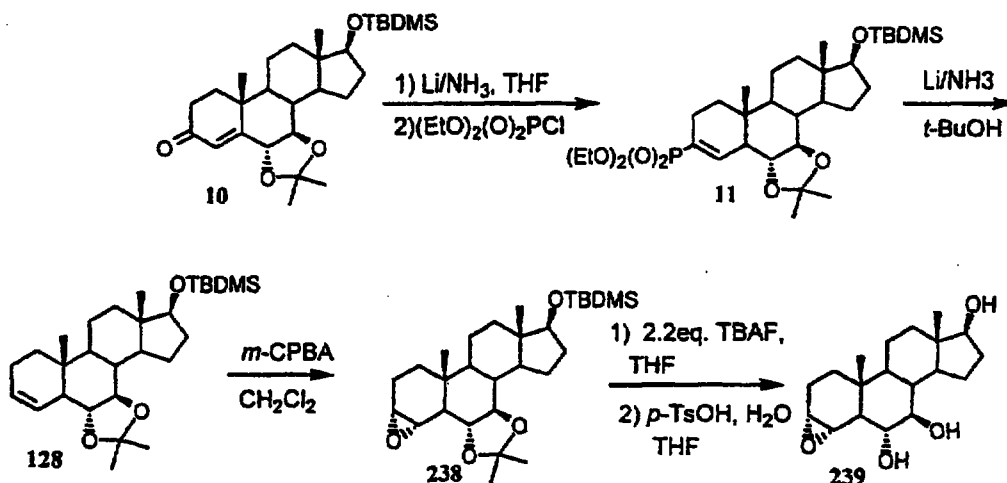
Scheme 60
