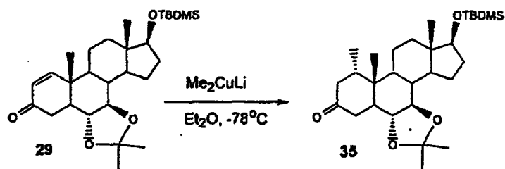
Scheme 8
