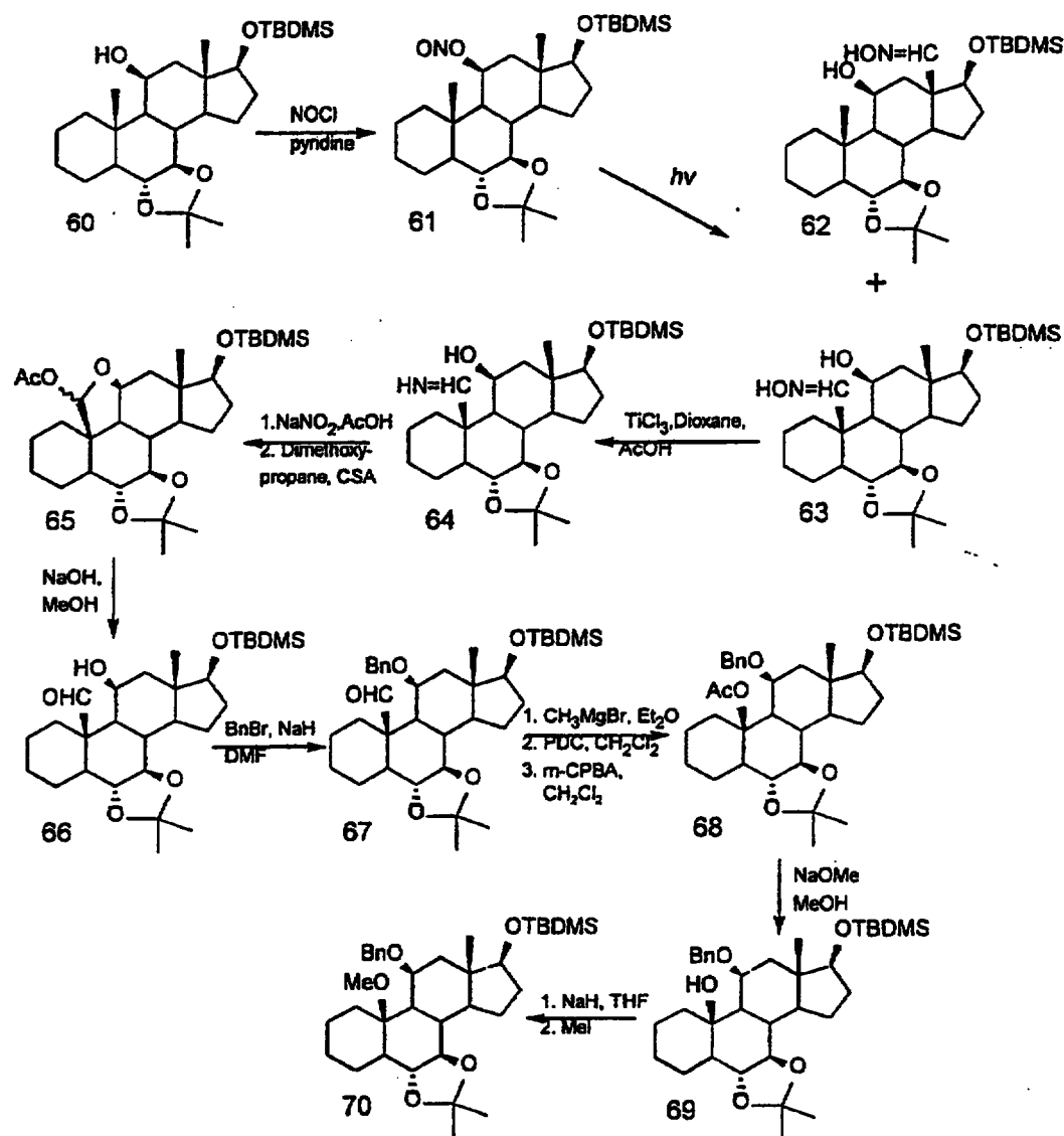
Scheme 20
