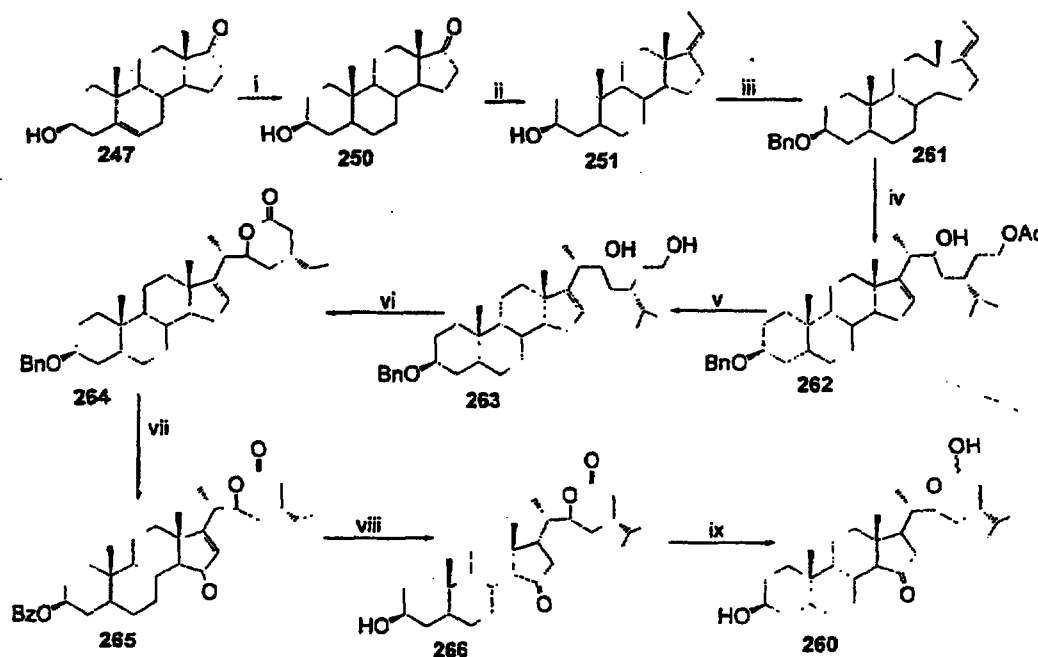
Scheme 65
