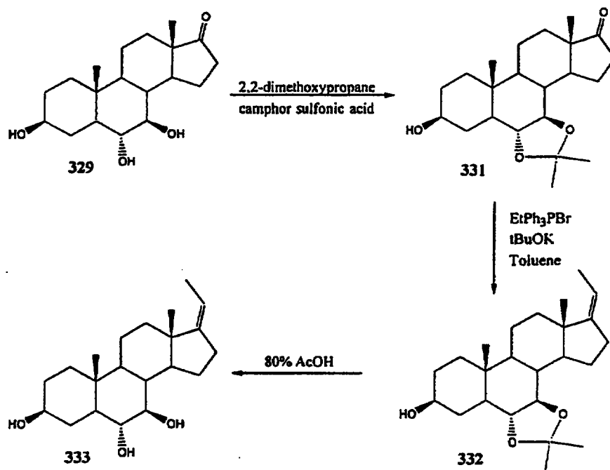
Scheme 80
