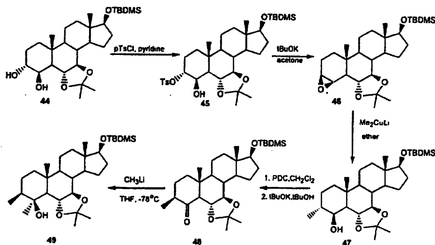
Scheme 13
