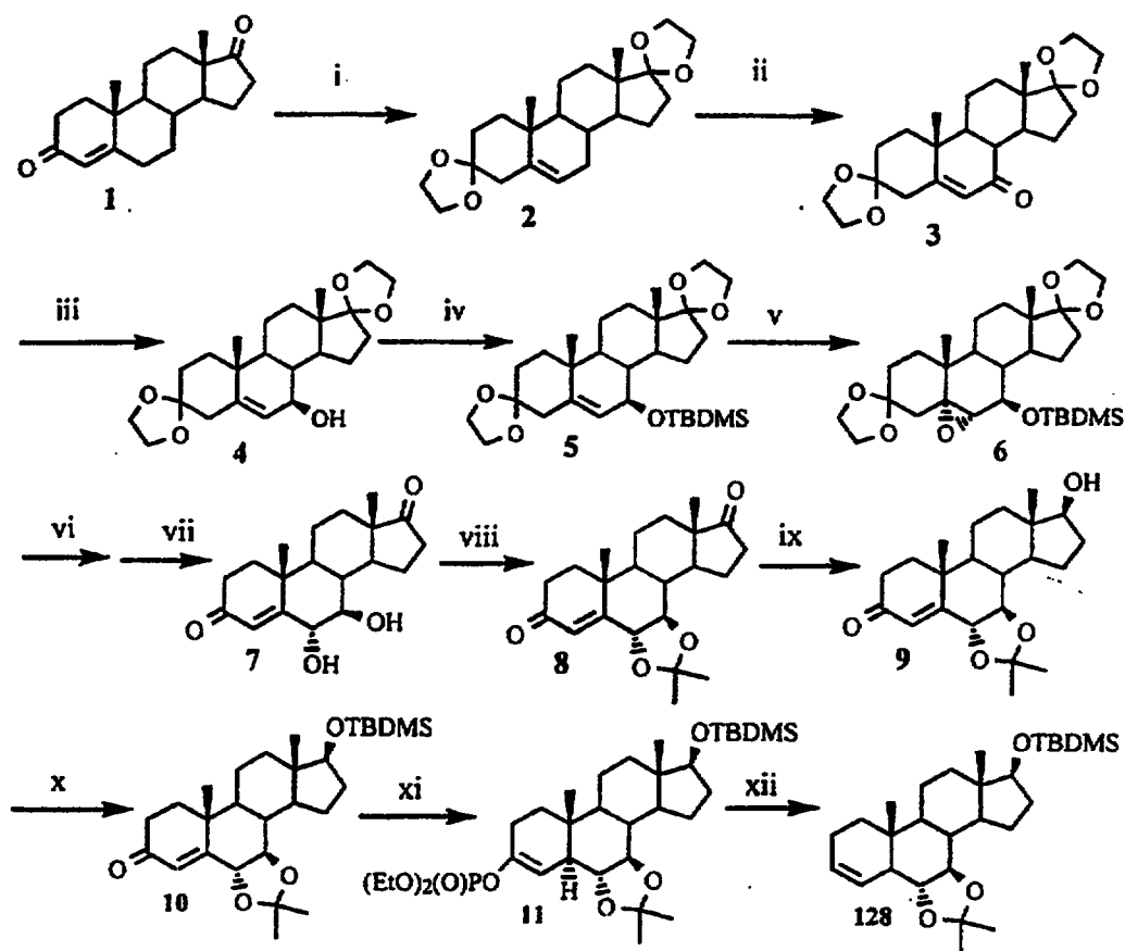
Scheme 75
