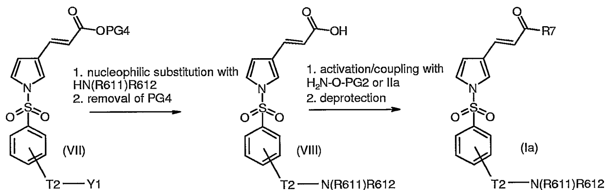
Reaction scheme 2:
