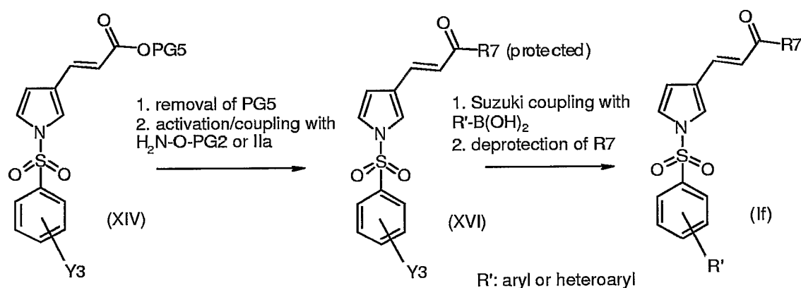
Reaction scheme 7:
