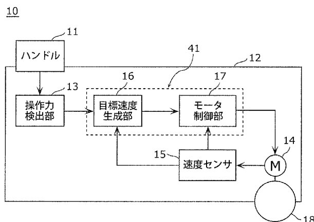
FIG. 1B: 11 Handlebar 13 Operation force detection unit 16 Target speed generation unit 17 Motor control unit 15 Speed sensor
