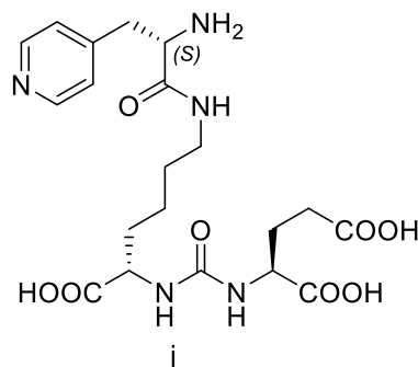
(((S)-5-(((S)-2-amino-3-(4-pyridinyl)propanamido)-1-carboxypentyl)carbamoyl)-L-glutamic acid
