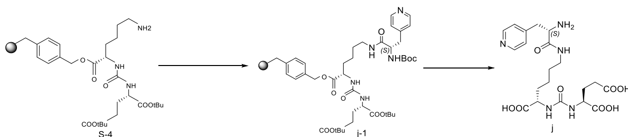
(((S)-5-(((S)-2-amino-3-(4-pyridinyl)propanamido)-1-carboxypentyl)carbamoyl)-L-glutamic acid
