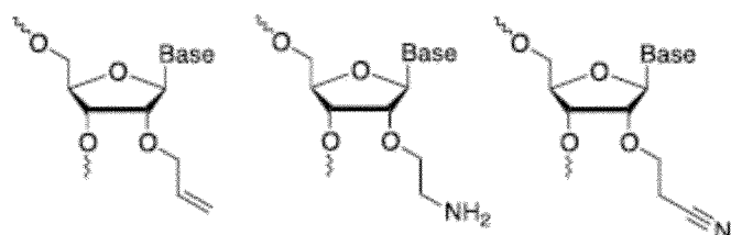
2'-O-Allyl
