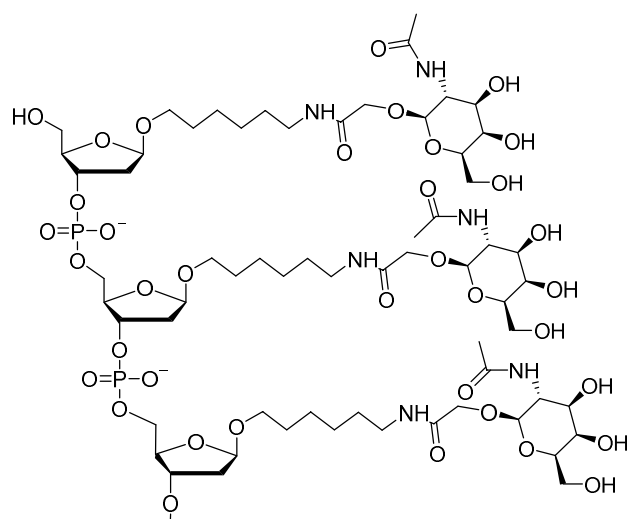
L53: Antisense strand of XD-06414 / Sense strand of XD-06414
