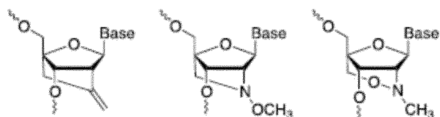
Methylene-clNA
