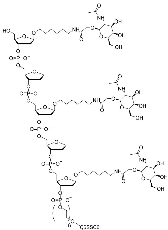
L19: Antisense strand of XD-06414 / Sense strand of XD-06414
