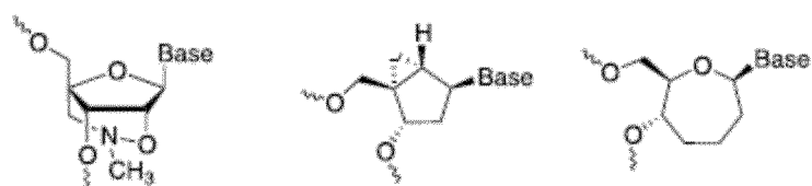
2',4'-BNANC[NMe]
