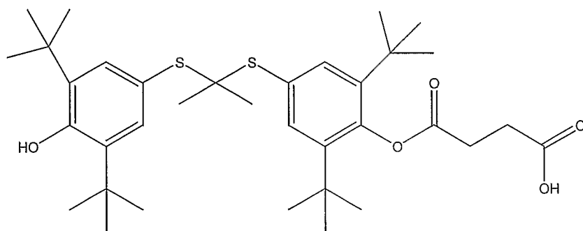
Compound A
