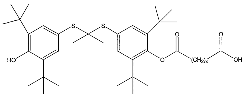
Formula I
