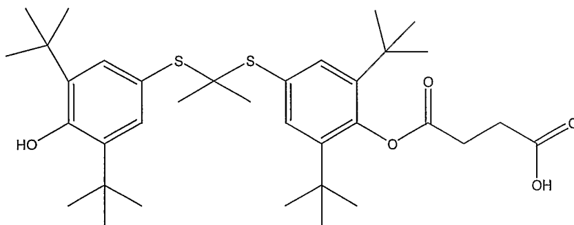
Compound A
