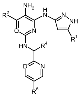
Formula (A);
