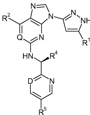
Formula (Ia)
