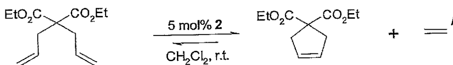
Scheme 4. RCM of diethyl diallylmalonate.
