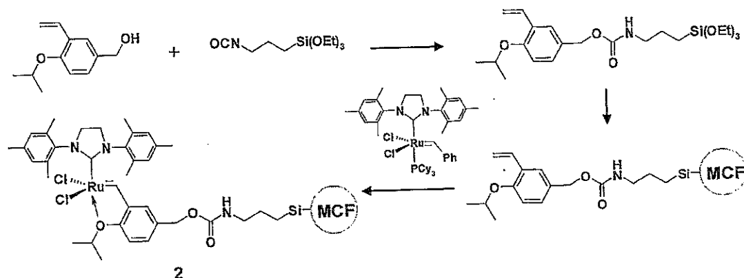
Scheme 3. Synthesis of MCF-supported Grubbs-Hoveyda catalyst.
