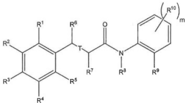
Formula (I)
