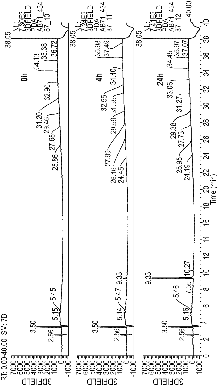
Fig. 23 UV- Chromatogram 380 nm
