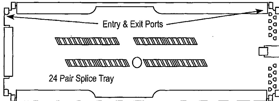
FIG. 4 Multi Fiber Splice Tray design for use with 24+ fiber designed cables
