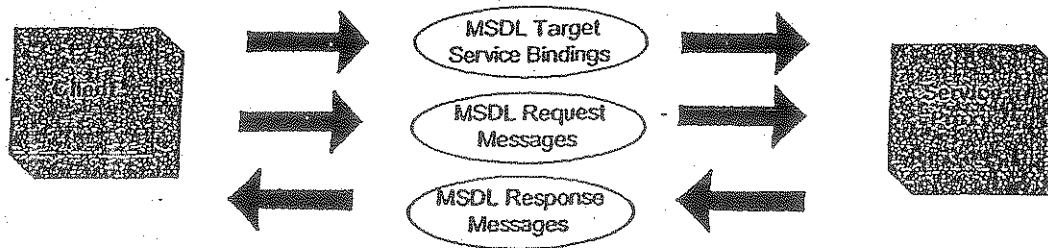
Service Proxy – Client Side MSDL Interaction Pattern
