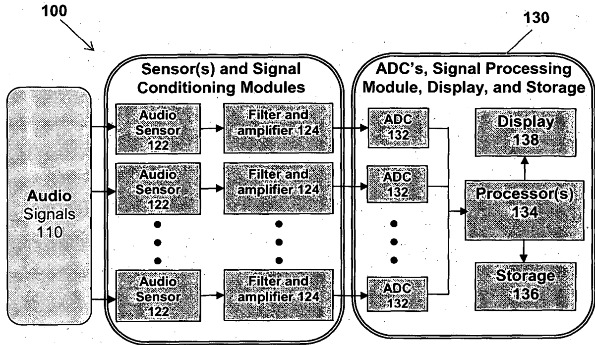
(a) Portable device configuration
