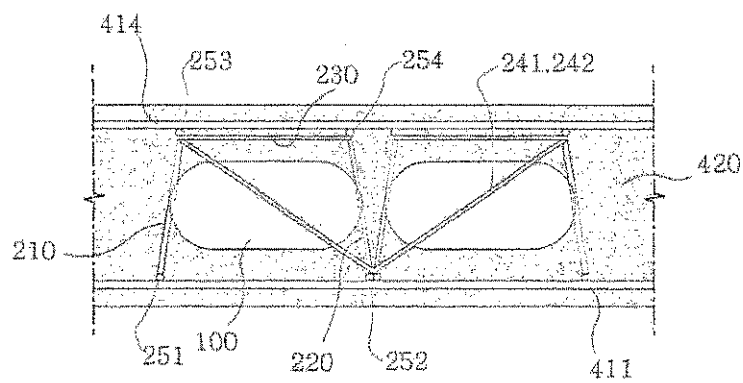
B-B Section
