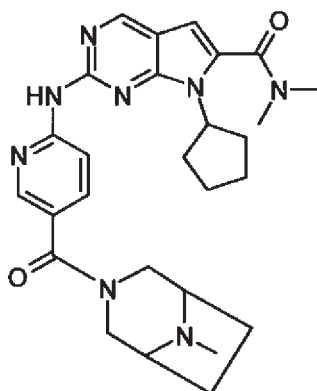
7-cyclopentyl-2-[5-(8-methyl-3,8-diaza-bicyclo[3.2.1]octane-3-carbonyl)-pyridin-2-ylamino]-7H-pyrrolo[2,3-d]pyrimidine-6-carboxylic acid dimethylamide
