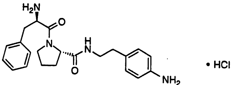
\text{D-Phe-Pro-p-NHCH}_2\text{CH}_2\text{C}_6\text{H}_4\text{NH}_2 \cdot \text{HCl}
