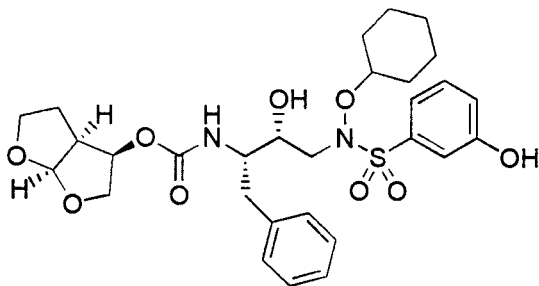
(3R,3aS,6aR)hexahydrofuro[2,3-b]furan-3-yl (1S,2R)-1-benzyl-3-[(cyclohexyloxy)[(3-hydroxyphenyl)sulfonyl]amino]-2-
