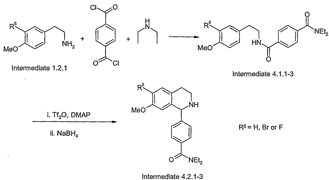
Scheme 4
