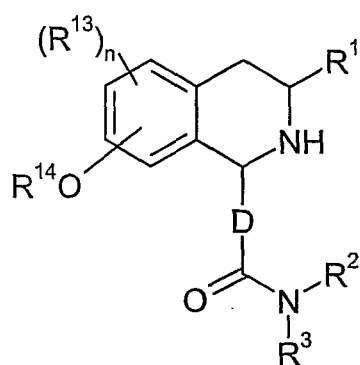
XI
