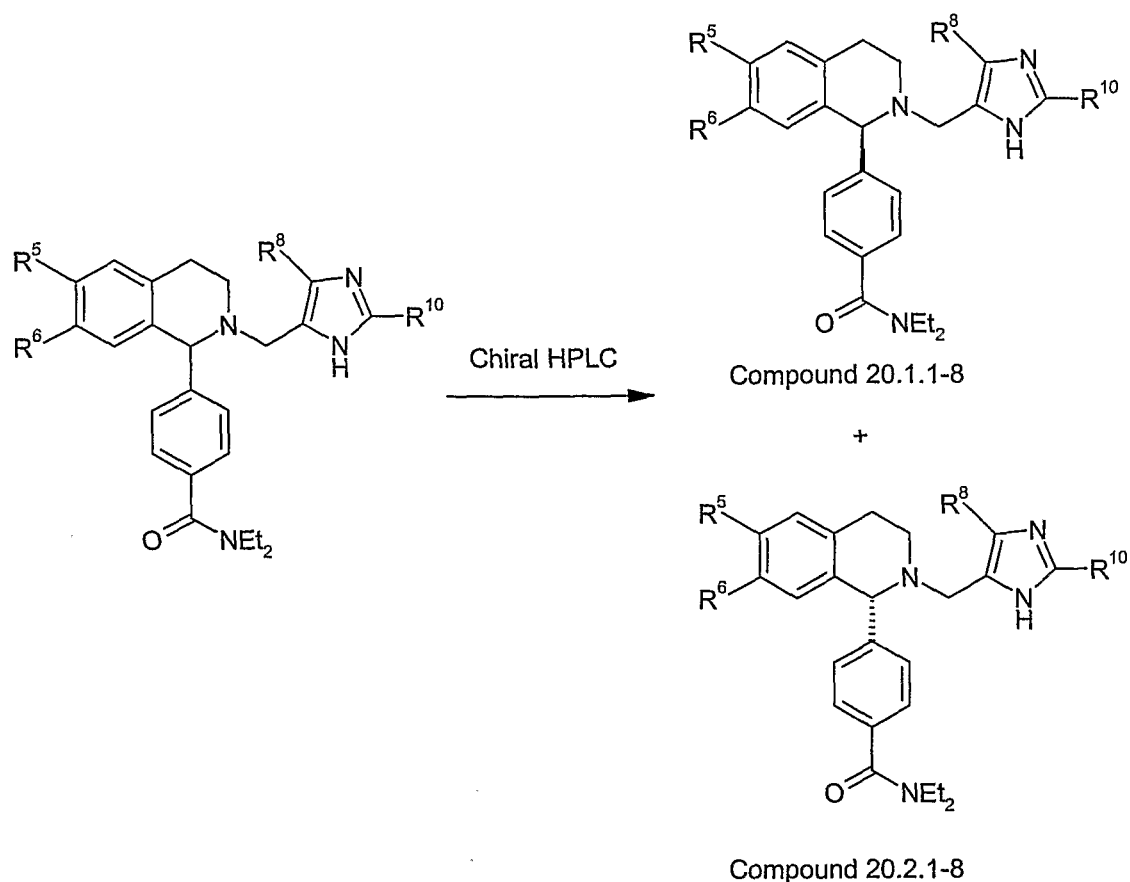
Scheme 20
