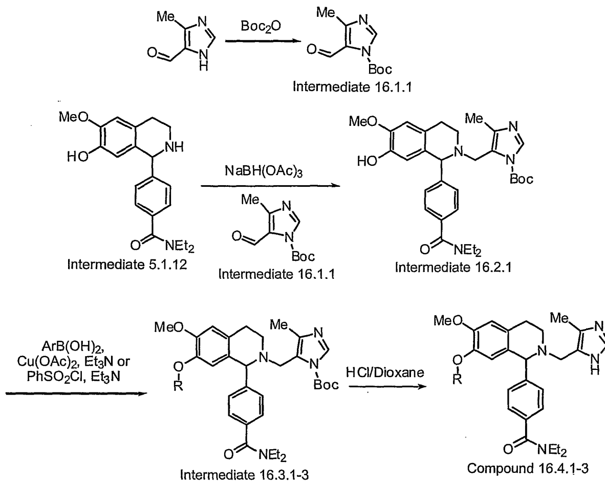
Scheme 16
