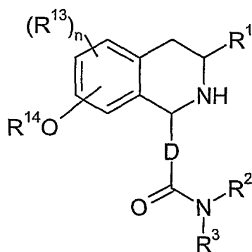
XI
