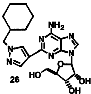
(4S,2R,3R,5R)-2-{6-amino-2-[1-(cyclohexylmethyl)pyrazol-4-yl]purin-9-yl}-5-(hydroxymethyl)oxolane-3,4-diol - 26
