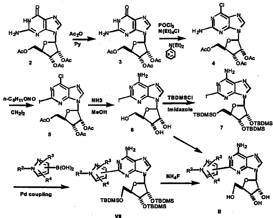
Scheme 3
