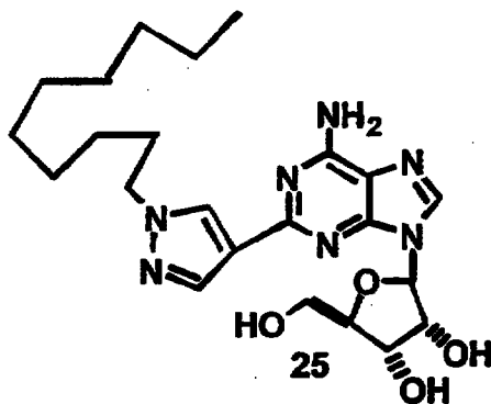
(4S,2R,3R,5R)-2-{6-amino-2-[1-decylpyrazol-4-yl]purin-9-yl}-5-(hydroxymethyl)oxolane-3,4-diol (25)
